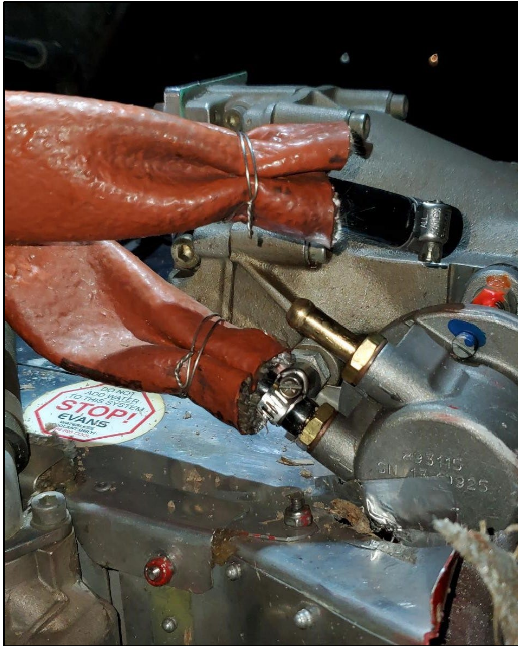
Photo 6 – Fuel Pump and Fuel Lines (FAA Photo)
