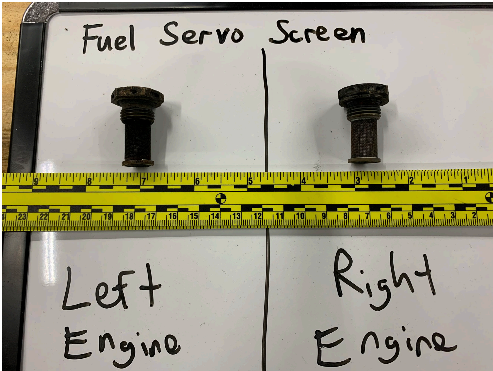
Photo 13 – View of the fuel servo screens for the left engine and the right engine.
