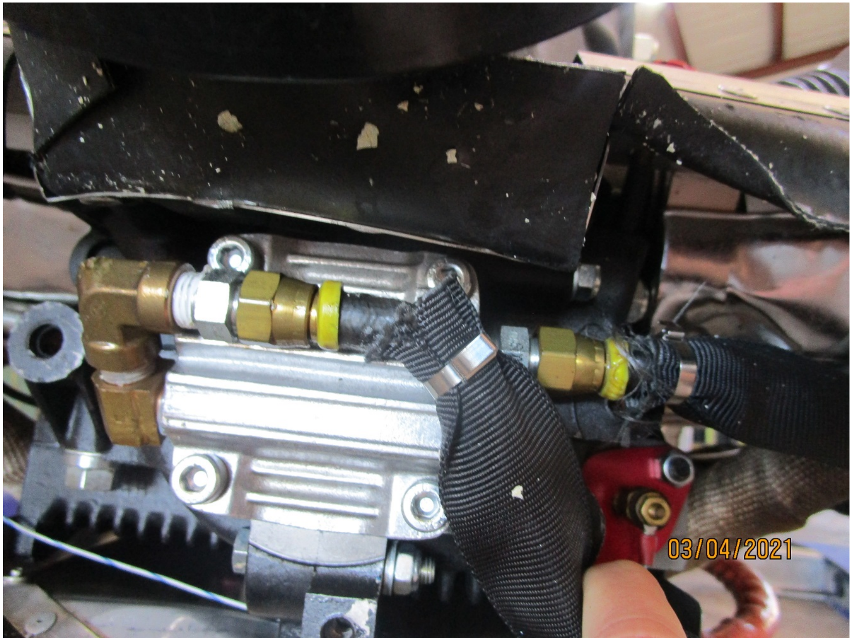
Photo 11 – Front of engine where oil filter lines connect
