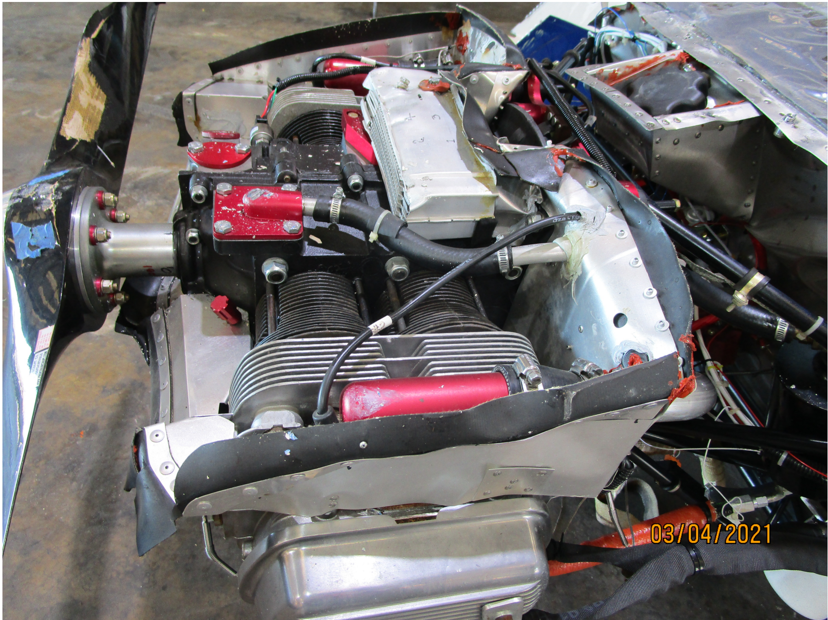
Photo 4 - Engine
