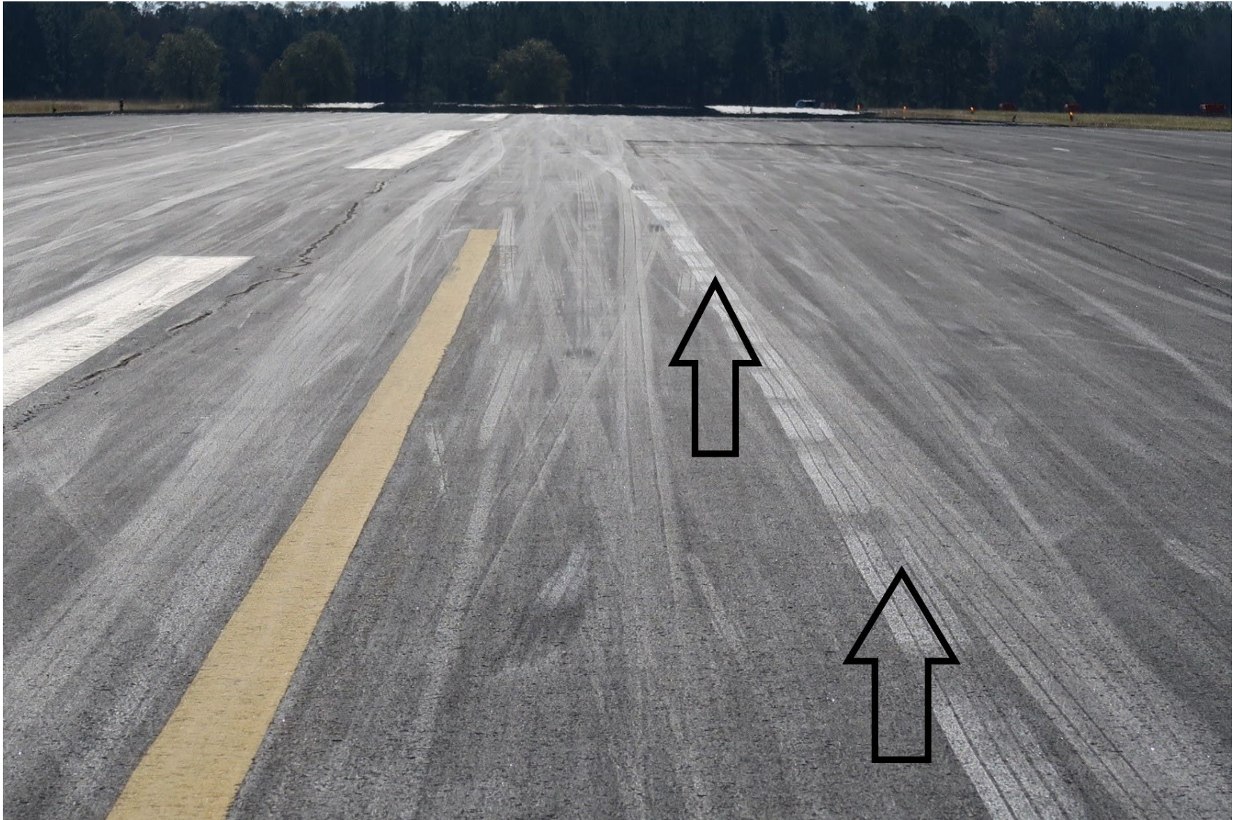
Photo 5 – Right Main Antiskid Marks on Runway 16 (Source: FAA)
