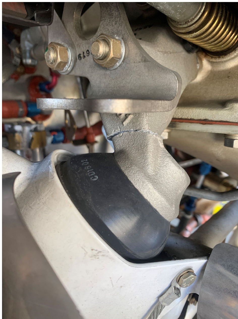
Photo 4 – View of the damaged engine mount (courtesy of the Federal Aviation Administration).
