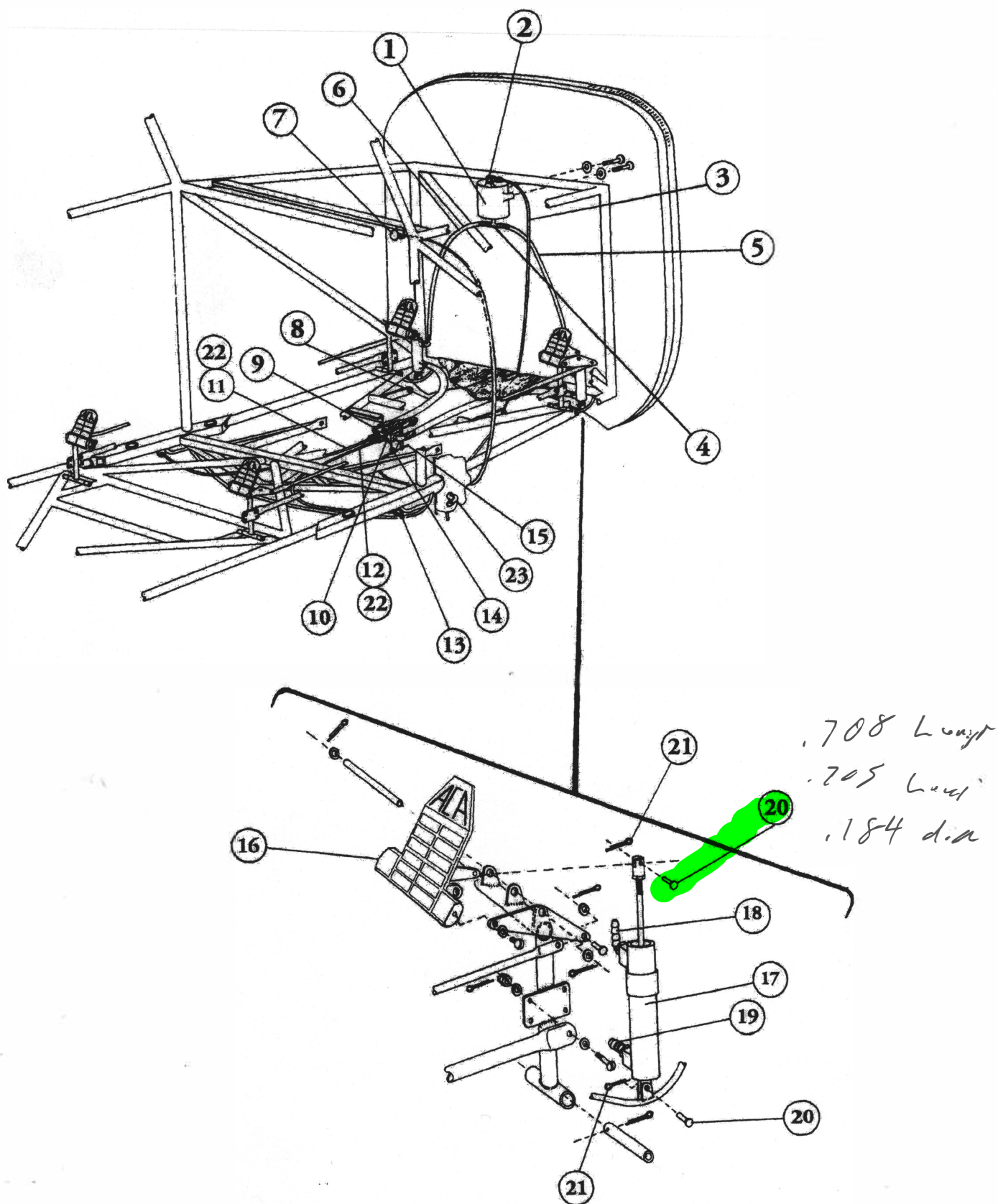
FIGURE 21 INSTALLATION - TOE BRAKE SYSTEM
