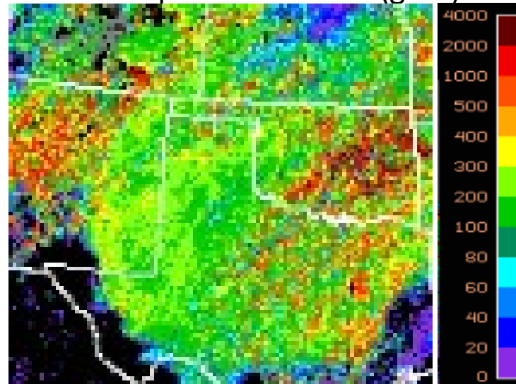
Liquid Water Path ( \text{gm}^{-2} )
