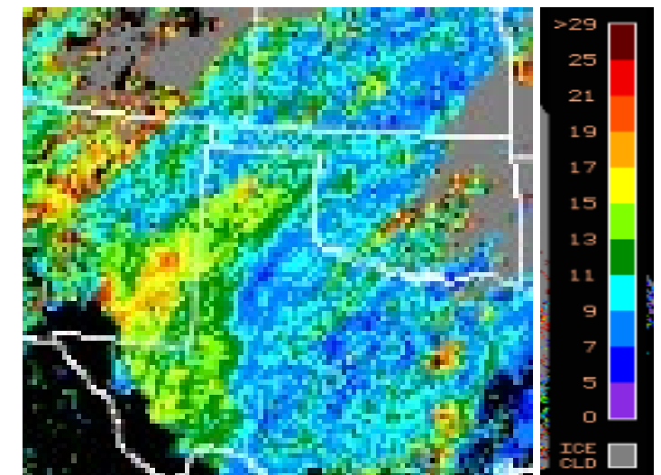
Water Cloud Effective Radius ( \mu\text{m} )
