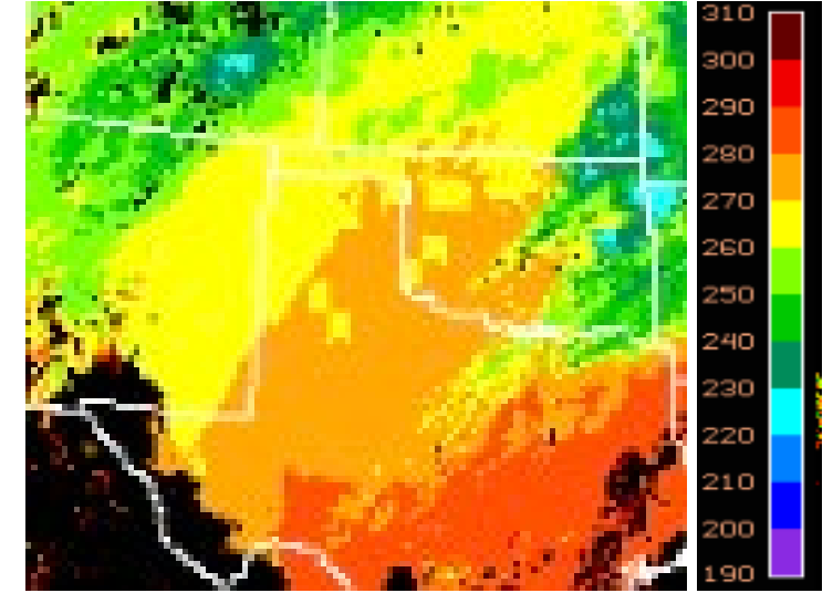
Cloud Temperature (K)
