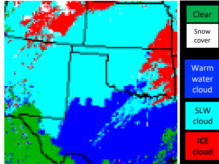
Cloud Top Phase
