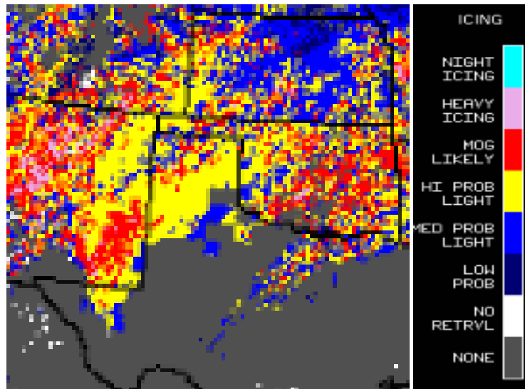
LaRC Satellite Flight Icing Threat
