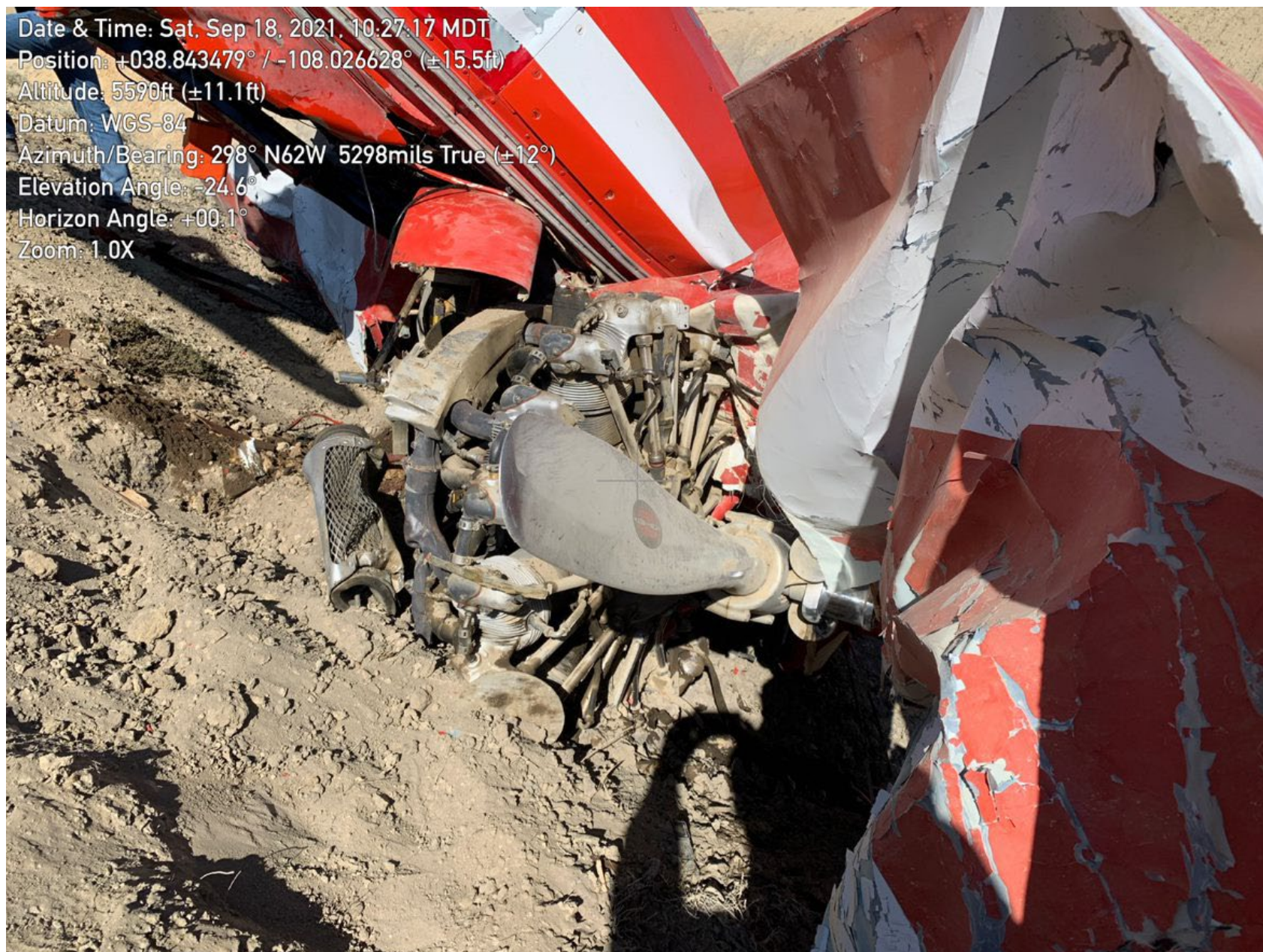
Photo 8 – Engine and Propeller Blade
