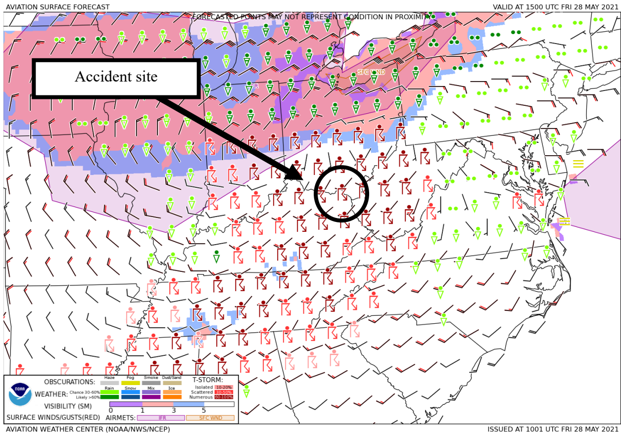
Figure 1 – GFA Surface Forecast valid at 1100 EDT with forecast issued at 0601 EDT.
