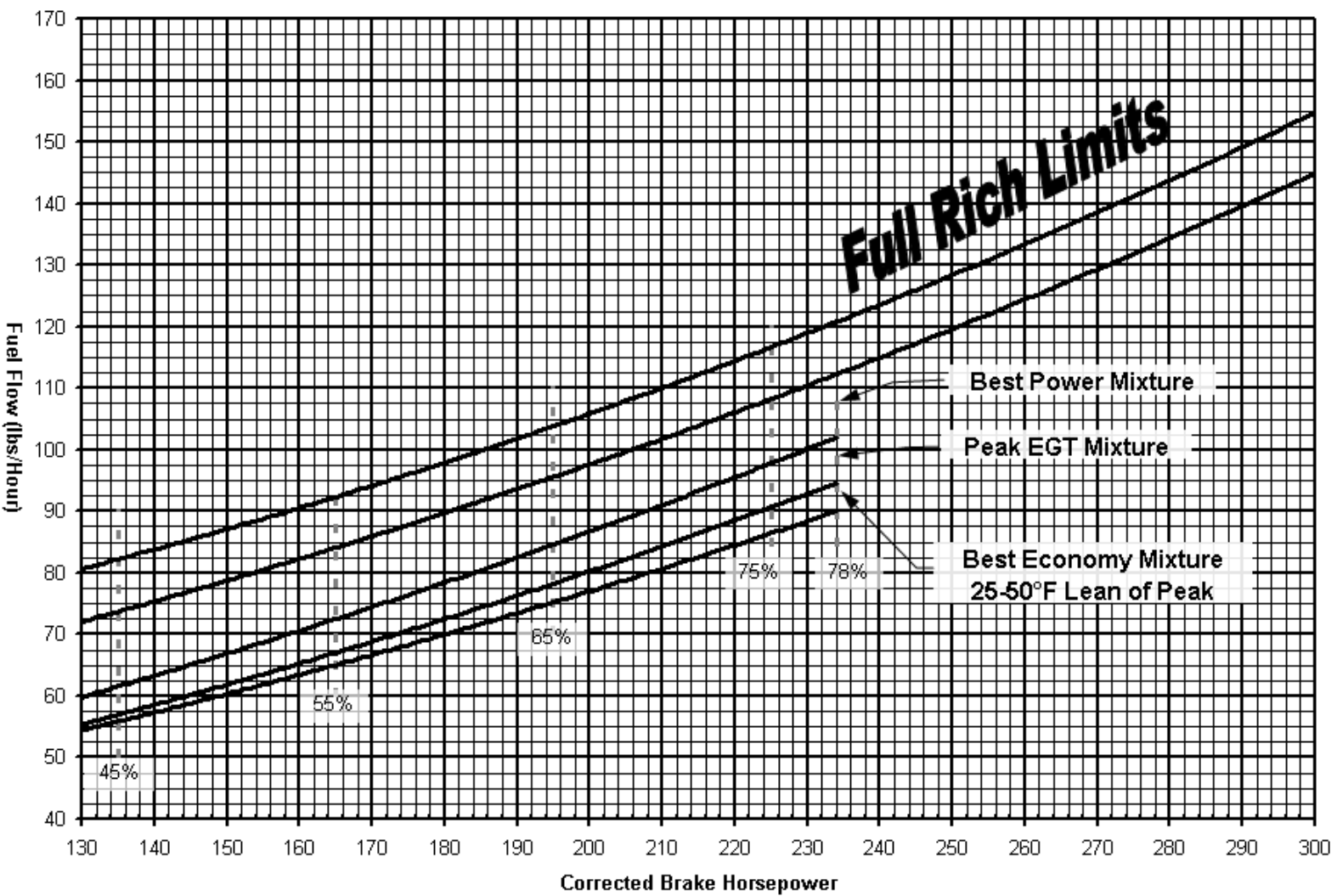
Figure 2-31. IO-550-B Fuel Flow vs. Brake Horsepower
