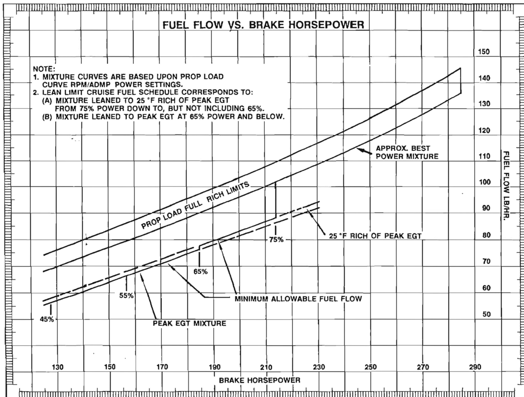
Figure 15-15-01. Fuel Flow Vs. BHP for IO-520-B, BA & BB
