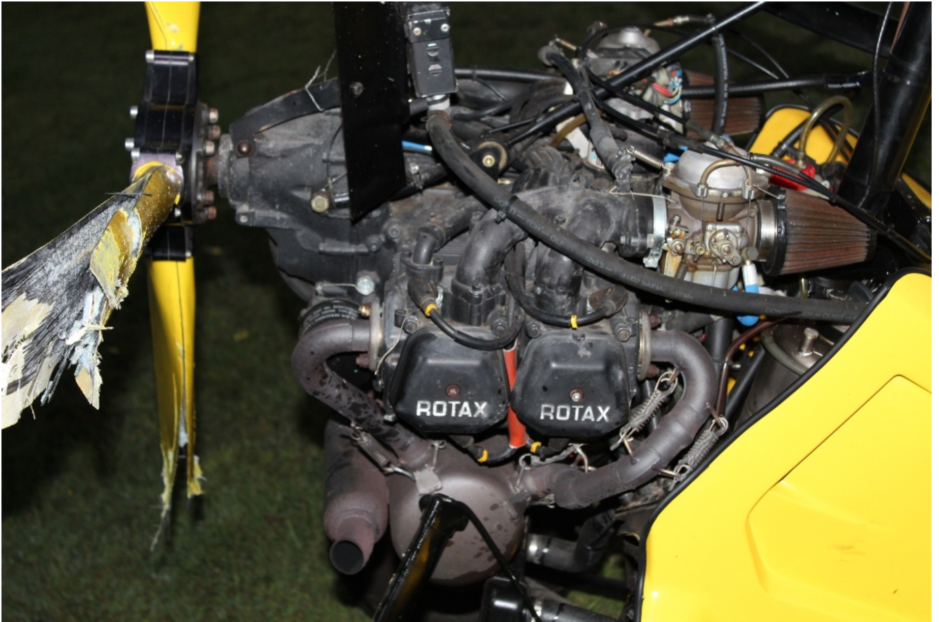
Photo 7 – View of the engine (courtesy of the Federal Aviation Administration).
