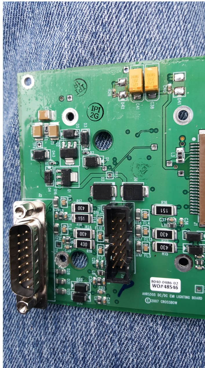
Photo 4 – Repaired Circuit Card
