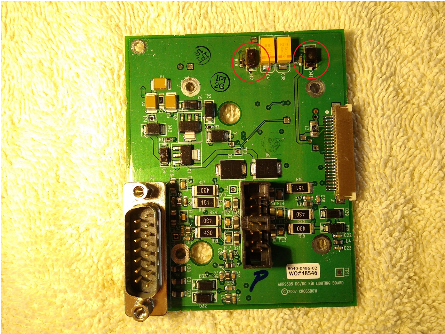
Photo 3 – Failed Circuit Card
