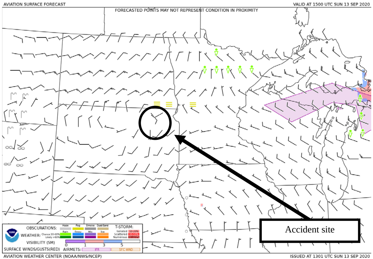
Figure 2 – GFA Surface Forecast valid at 1000 CDT with forecast issued at 0801 CDT
