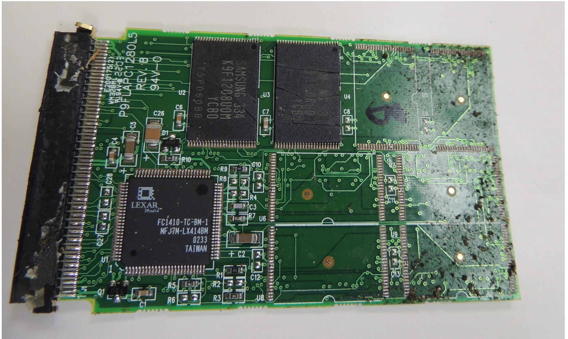
Photo 9 - Supplied view of the compact flash exhibiting cracked NVM.
