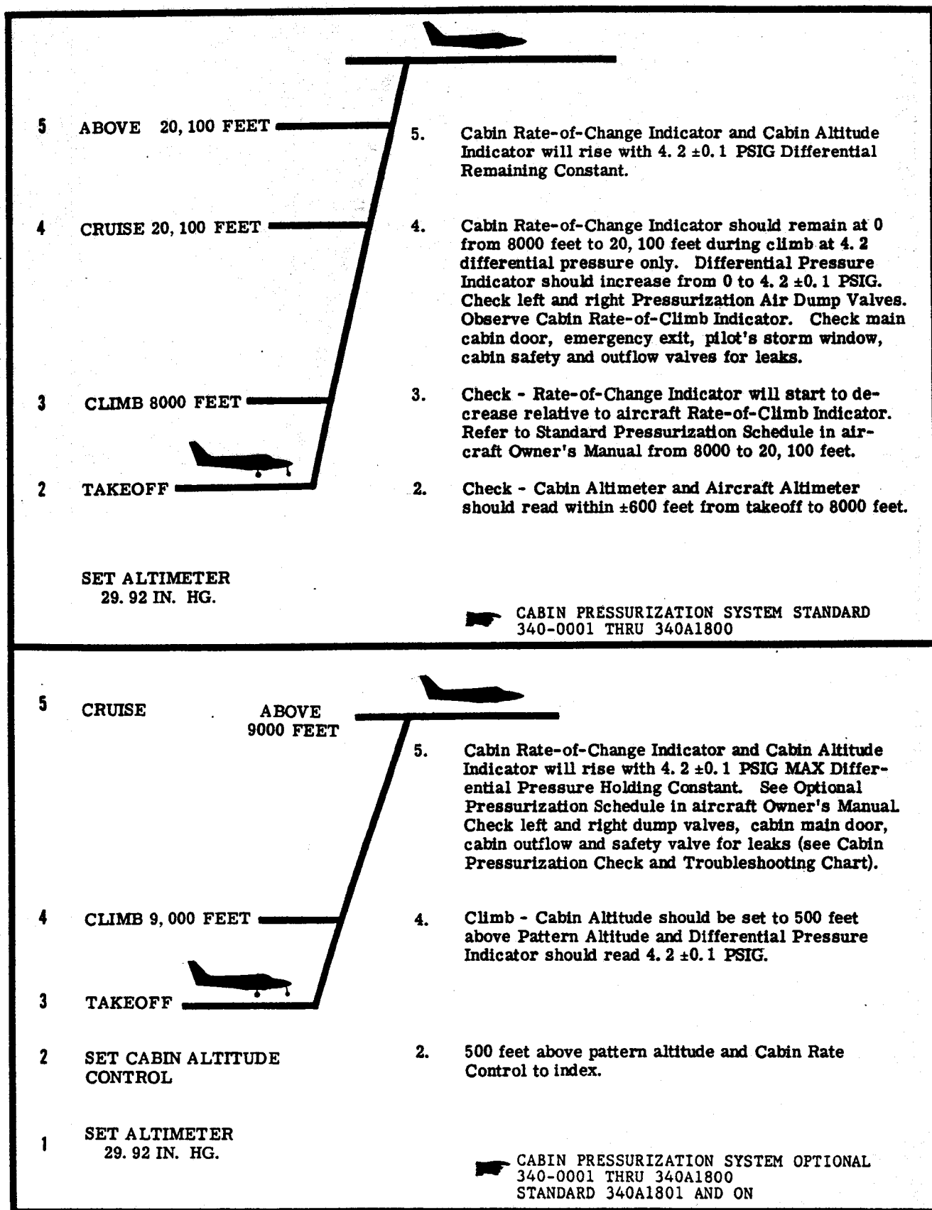
Figure 13-10. Cabin Pressurization Operation Flight Check Chart
