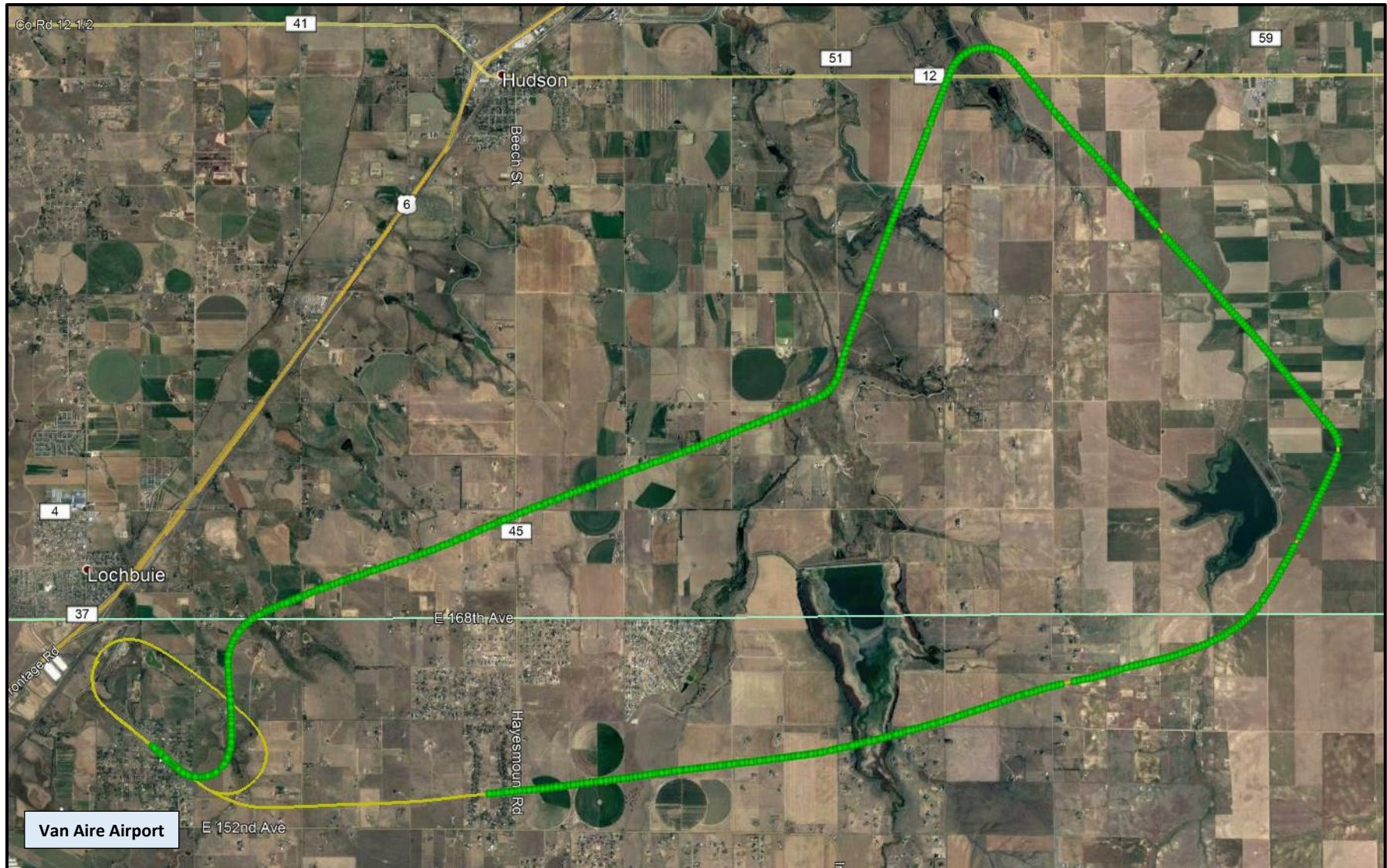
Figure 2 – Initial takeoff until return to airport (1157 mdt ~ 1208 mdt)
