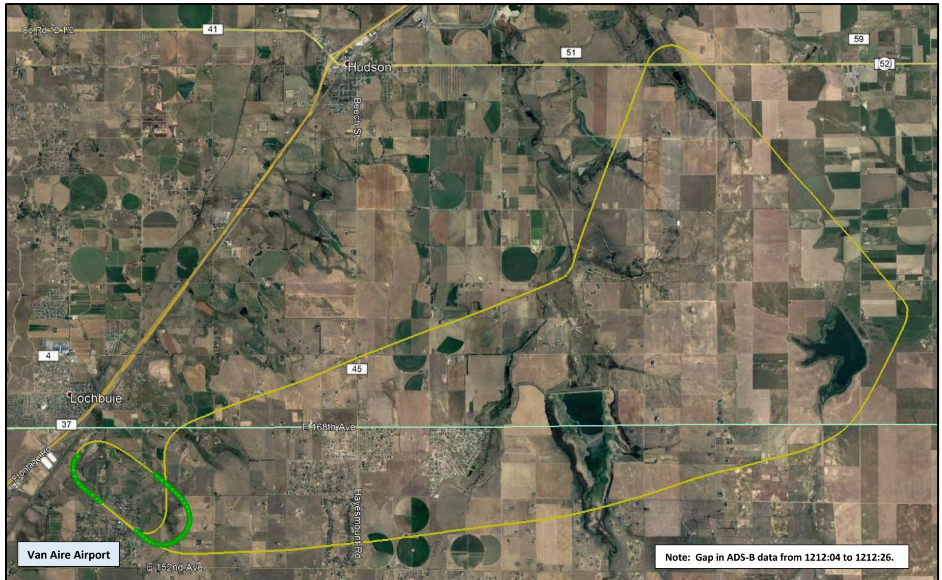
Figure 4 – Accident touch-and-go (1211 mdt ~ 1213 mdt)
