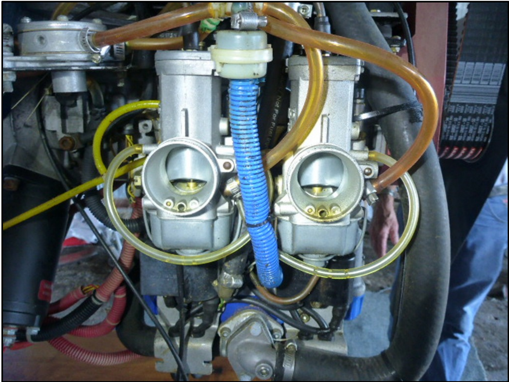
Photo 7 – Engine (Rotech Photo)
