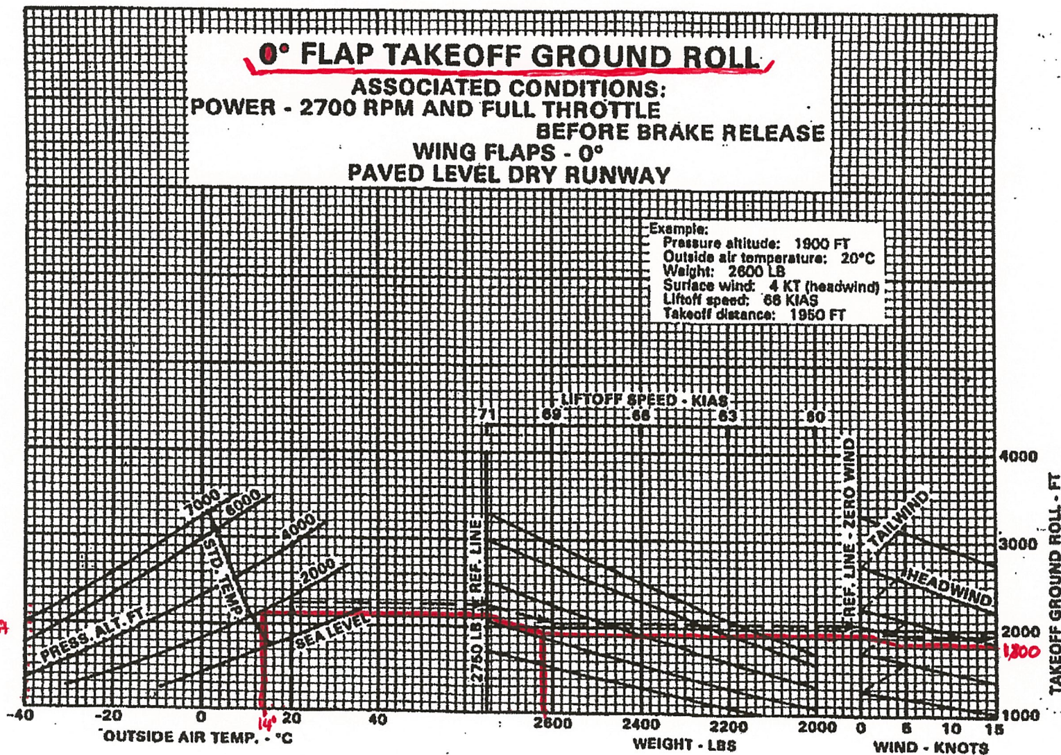
0° FLAP TAKEOFF GROUND ROLL Figure 5-15
