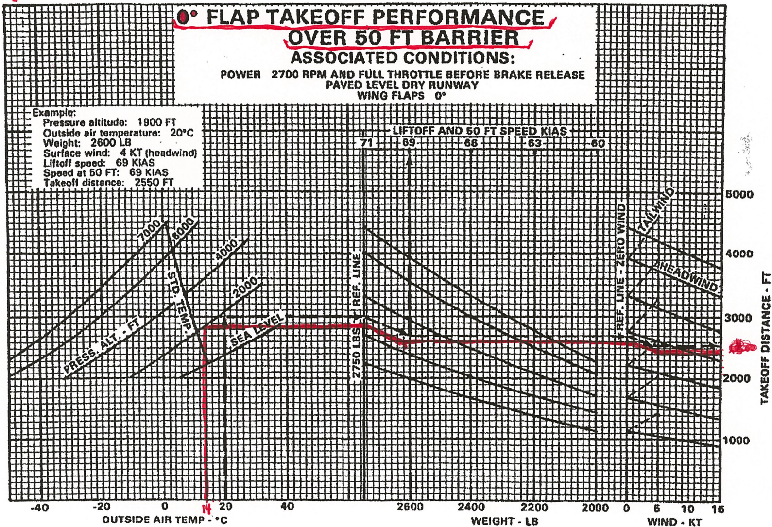
0° FLAP TAKEOFF PERFORMANCE Figure 5-13
