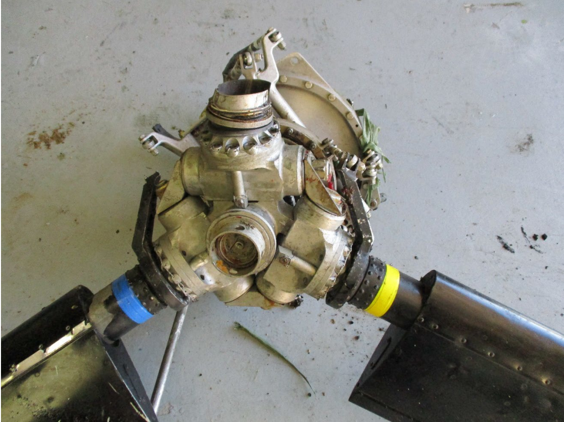
Photo 4: Main Rotor Assembly (Source – Federal Aviation Administration)
