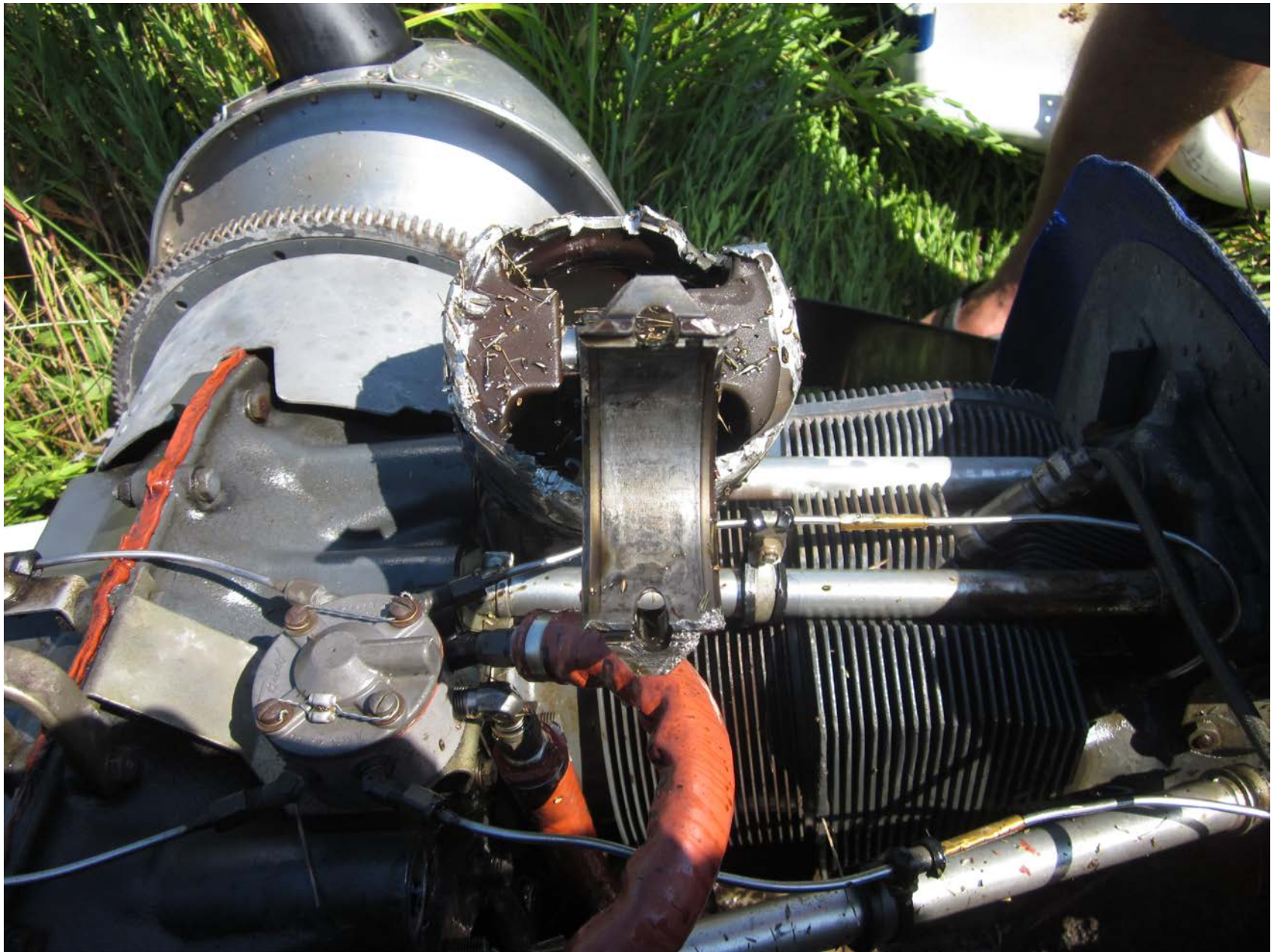
Photo 5 – Separated Piston and Fractured Connecting Rod (FAA)
