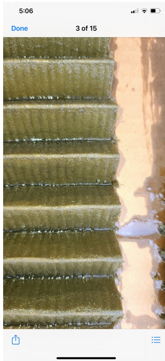
Photo 6 – View of the cut open engine oil filter (courtesy of Wentworth Aircraft, Inc.).
