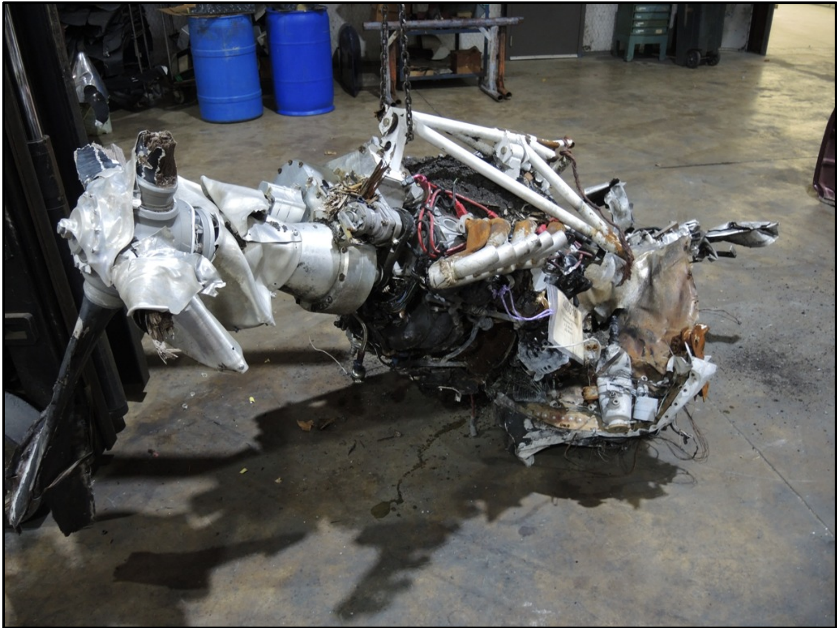
Photo 3 – Engine / Propeller
