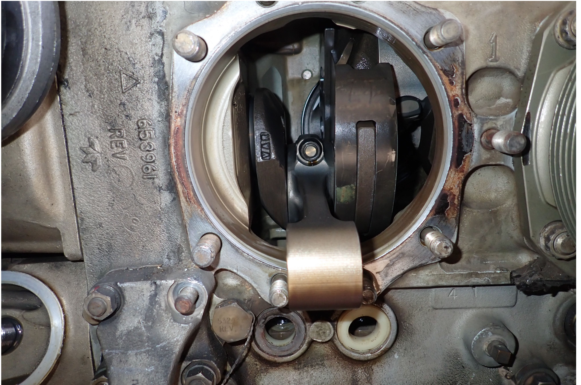
Photo 5 – No. 1 Connecting Rod
