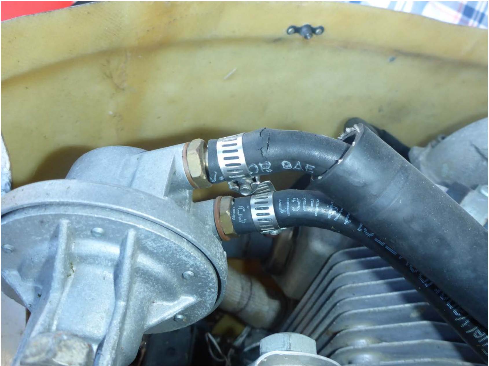
Photo 4 – Fuel Lines (Rotech Photo)
