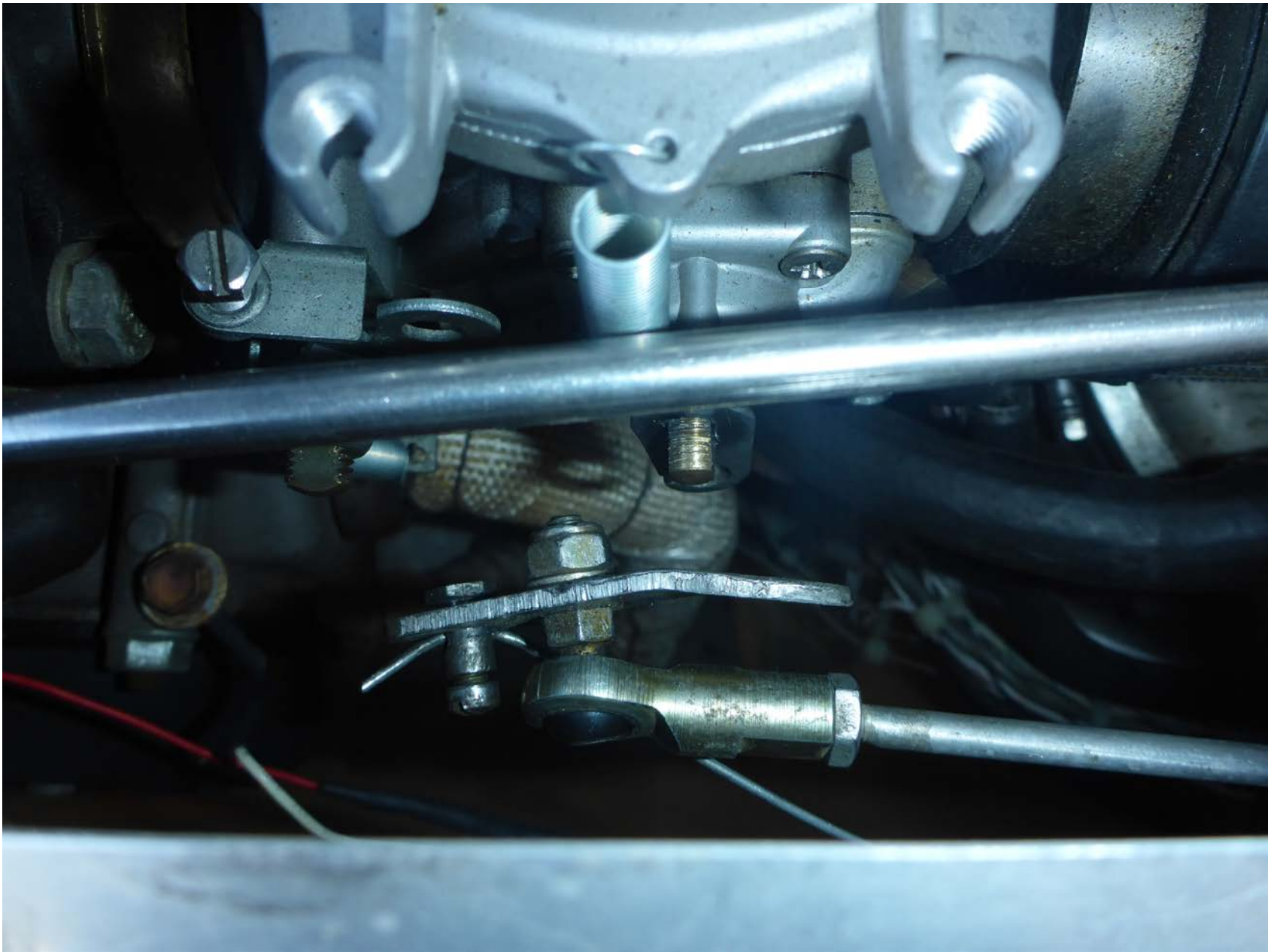
Photo 2 – Disconnected Choke Lever (Rotech Photo)
