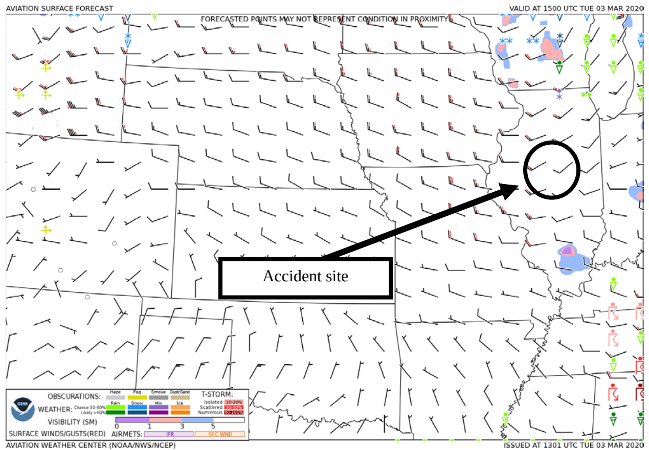
Figure 2 – GFA Surface Forecast valid at 0900 CST with forecast issued at 0701 CST
