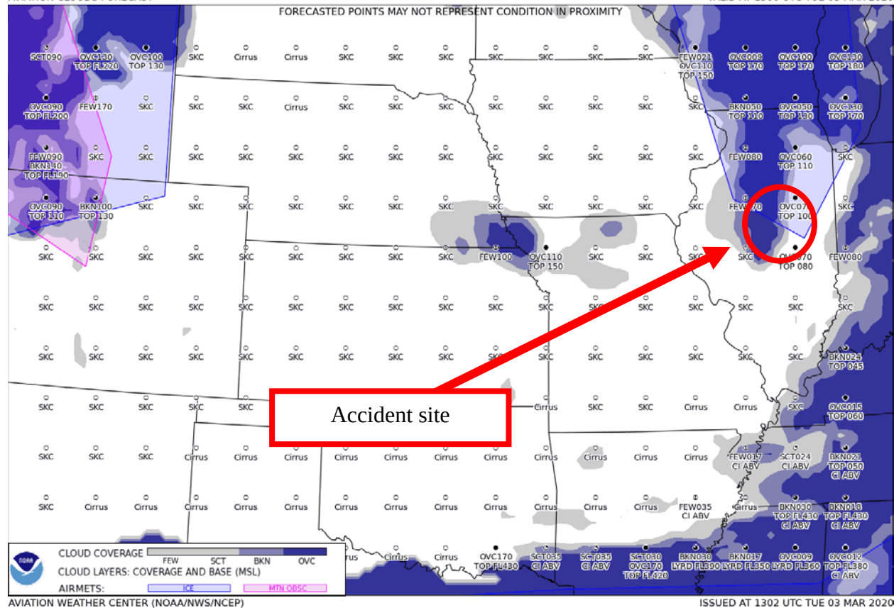
Figure 4 – GFA Aviation Clouds Forecast valid at 0900 CST with forecast issued at 0702 CST
