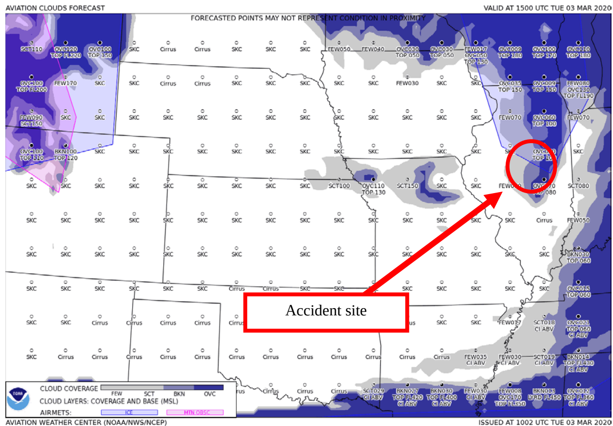
Figure 3 – GFA Aviation Clouds Forecast valid at 0900 CST with forecast issued at 0402 CST
