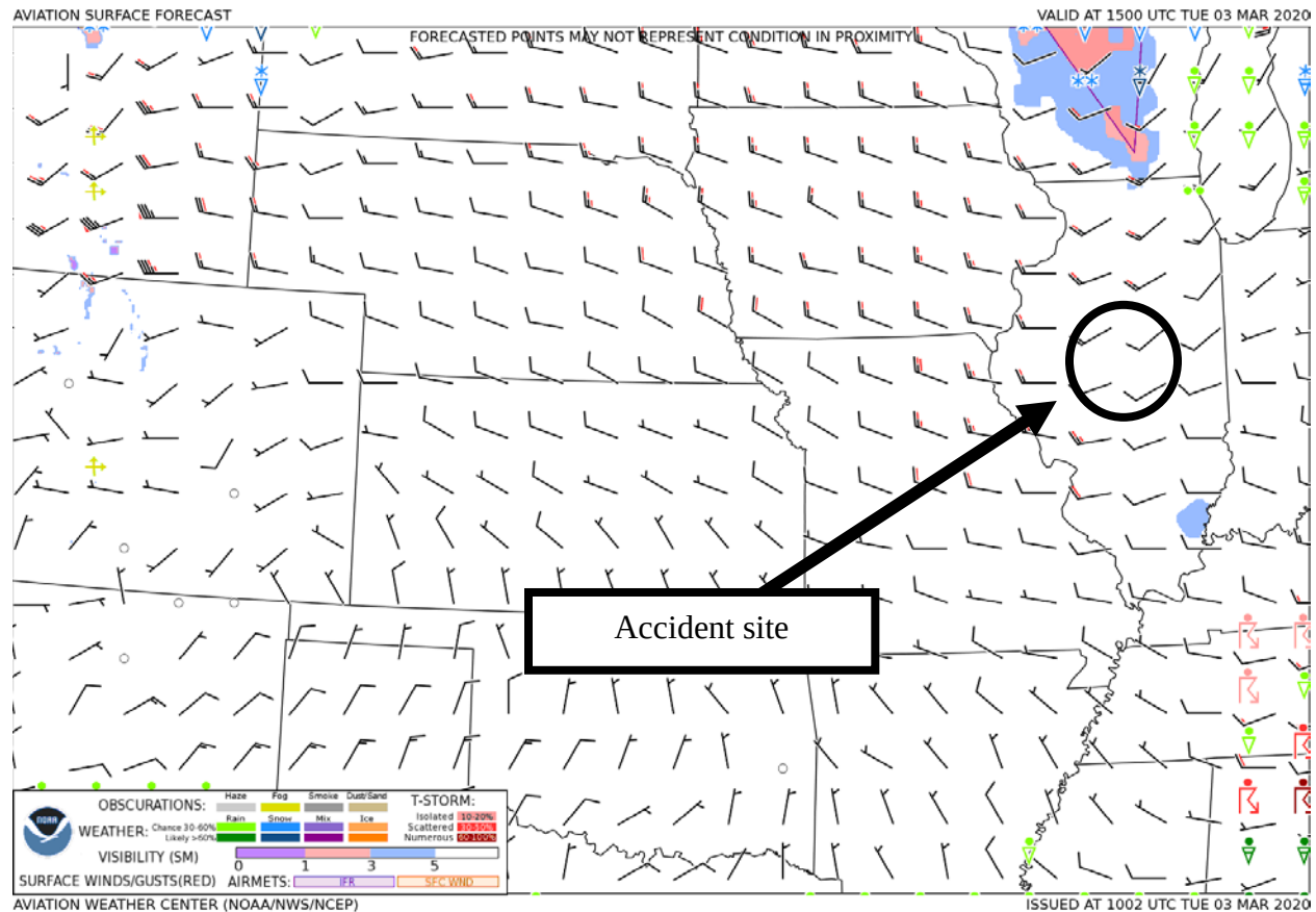
Figure 1 – GFA Surface Forecast valid at 0900 CST with forecast issued at 0402 CST
