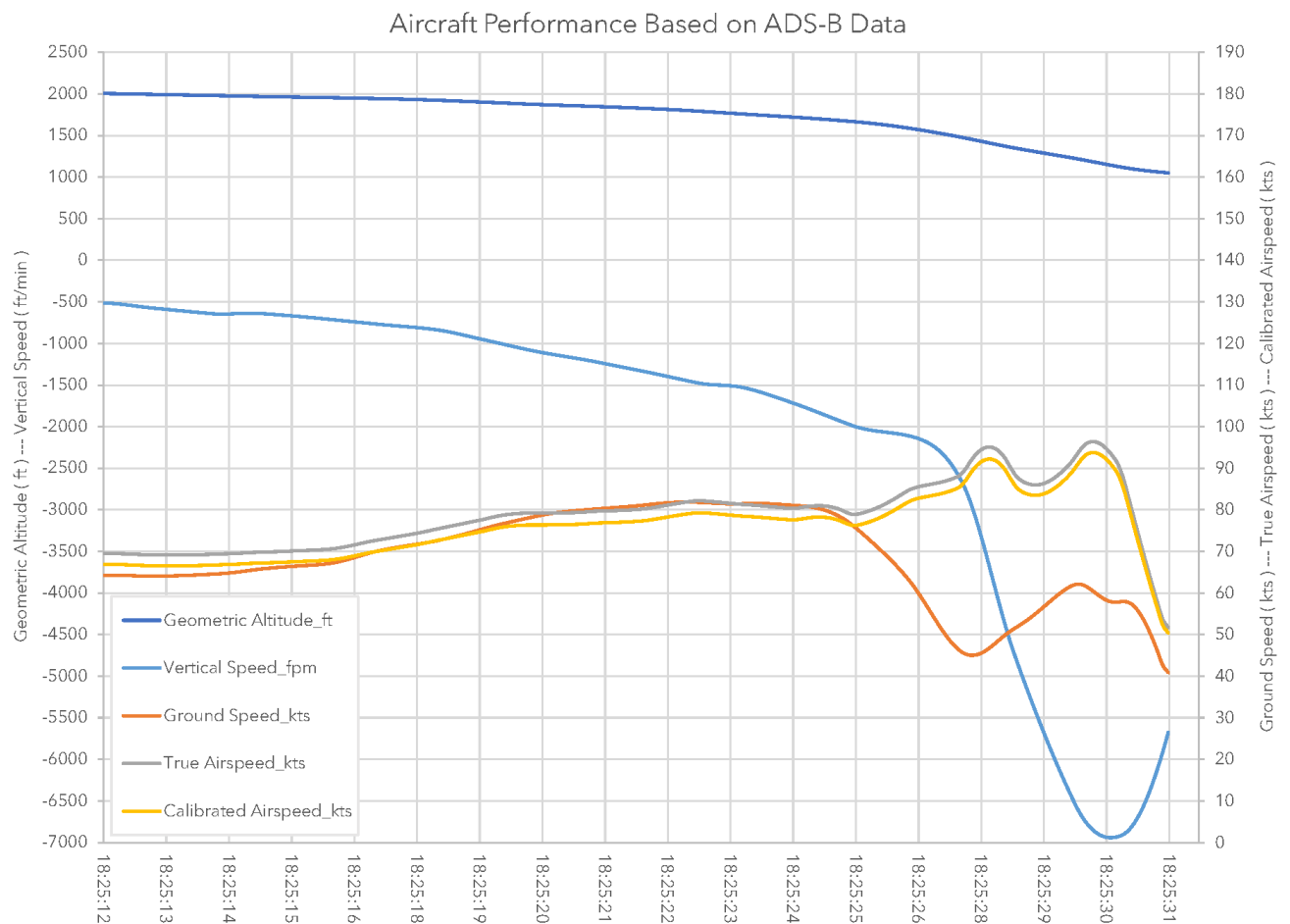
Figure 1 Airplane Performance
