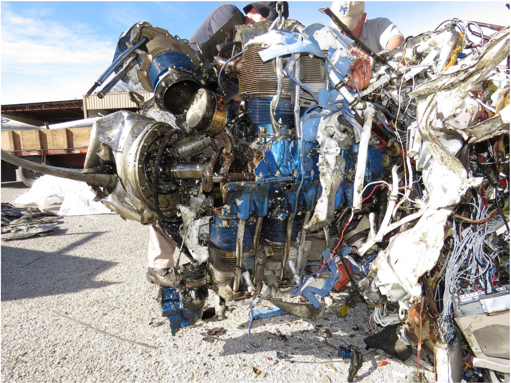
Photo 6 – Engine (Lycoming Photo)
