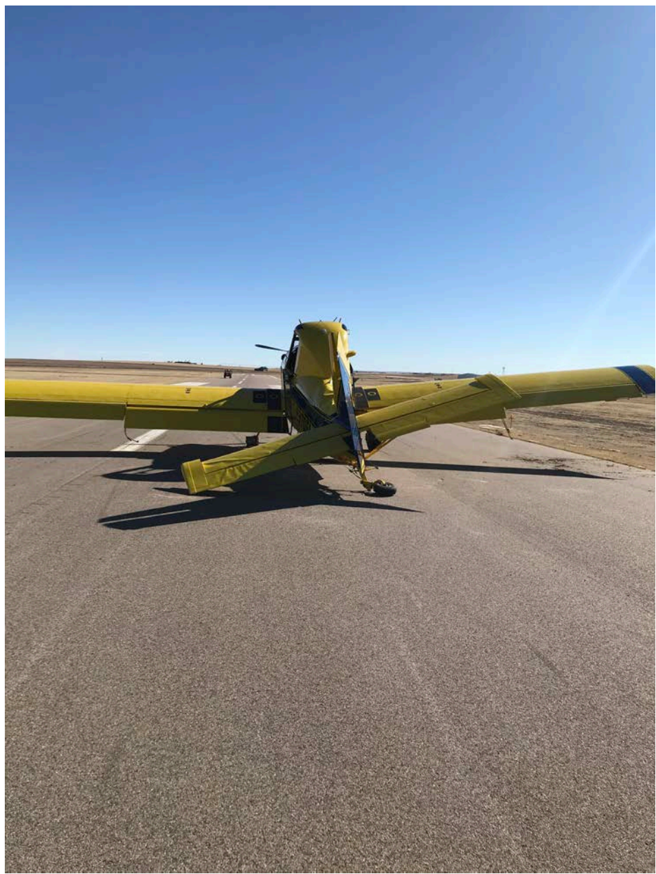
Photo 2 – View of damage to the elevator and horizontal stabilizer (Courtesy of FAA)
