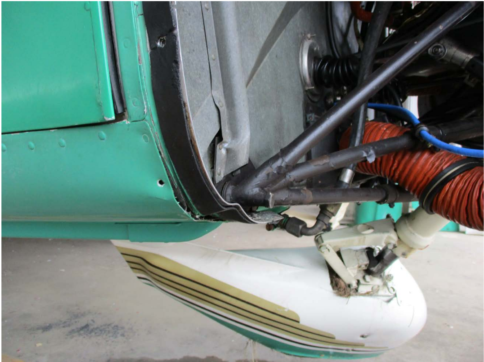
Photo 1 – View of damage to the engine mounts (Courtesy of FAA)
