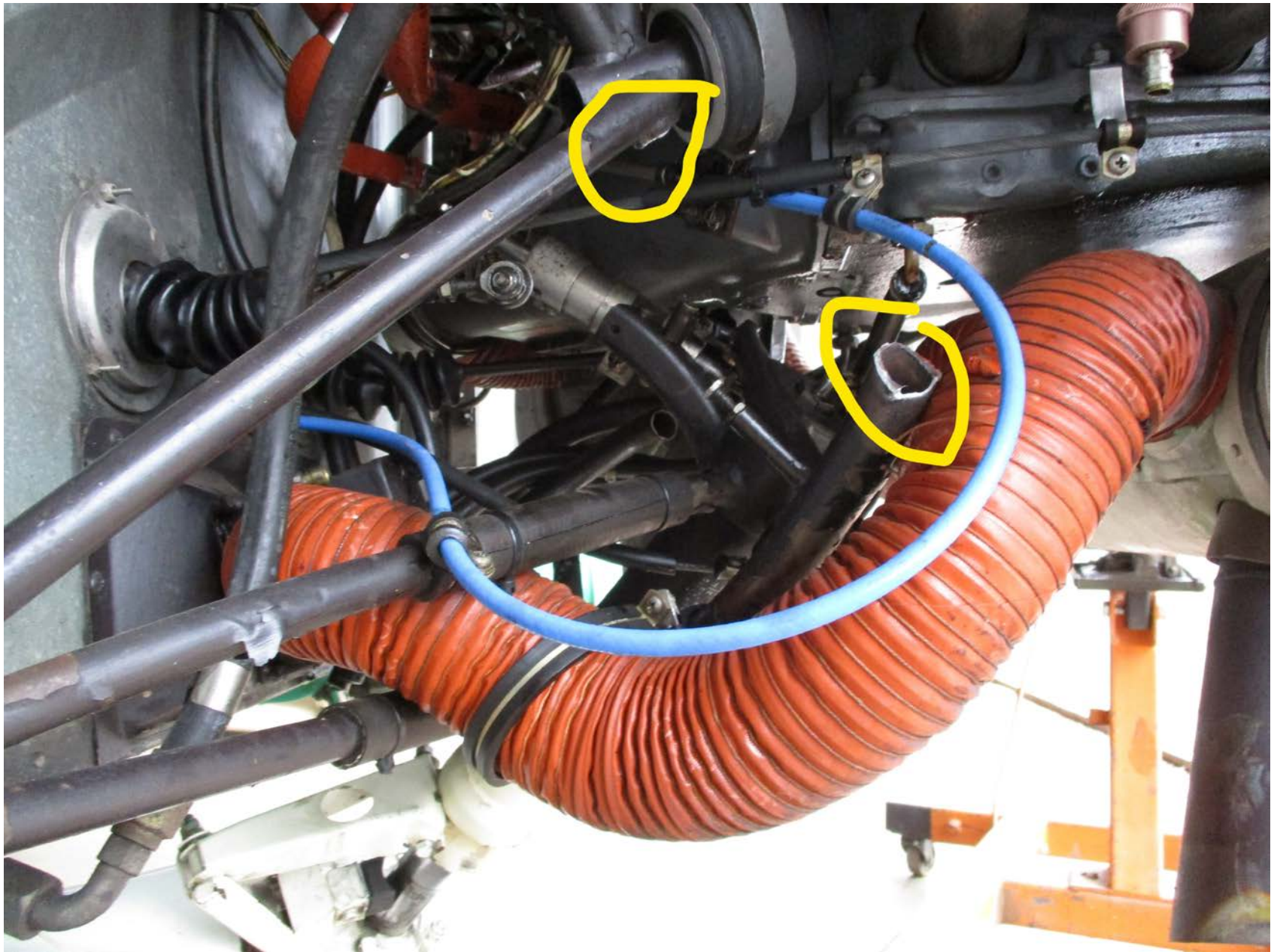
Photo 2 – View of damage to the engine mounts (Courtesy of FAA)
