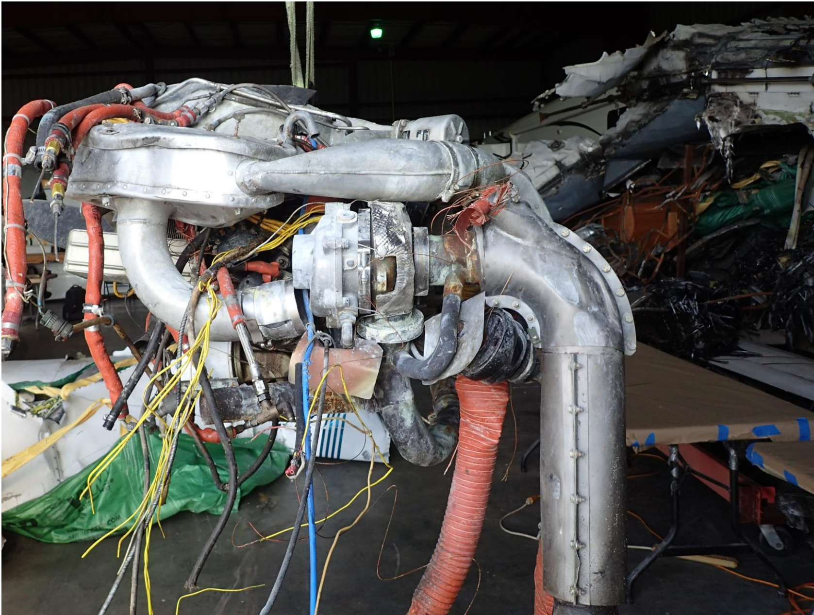
Photo 8 – Turbocharger (CAT Photo)
