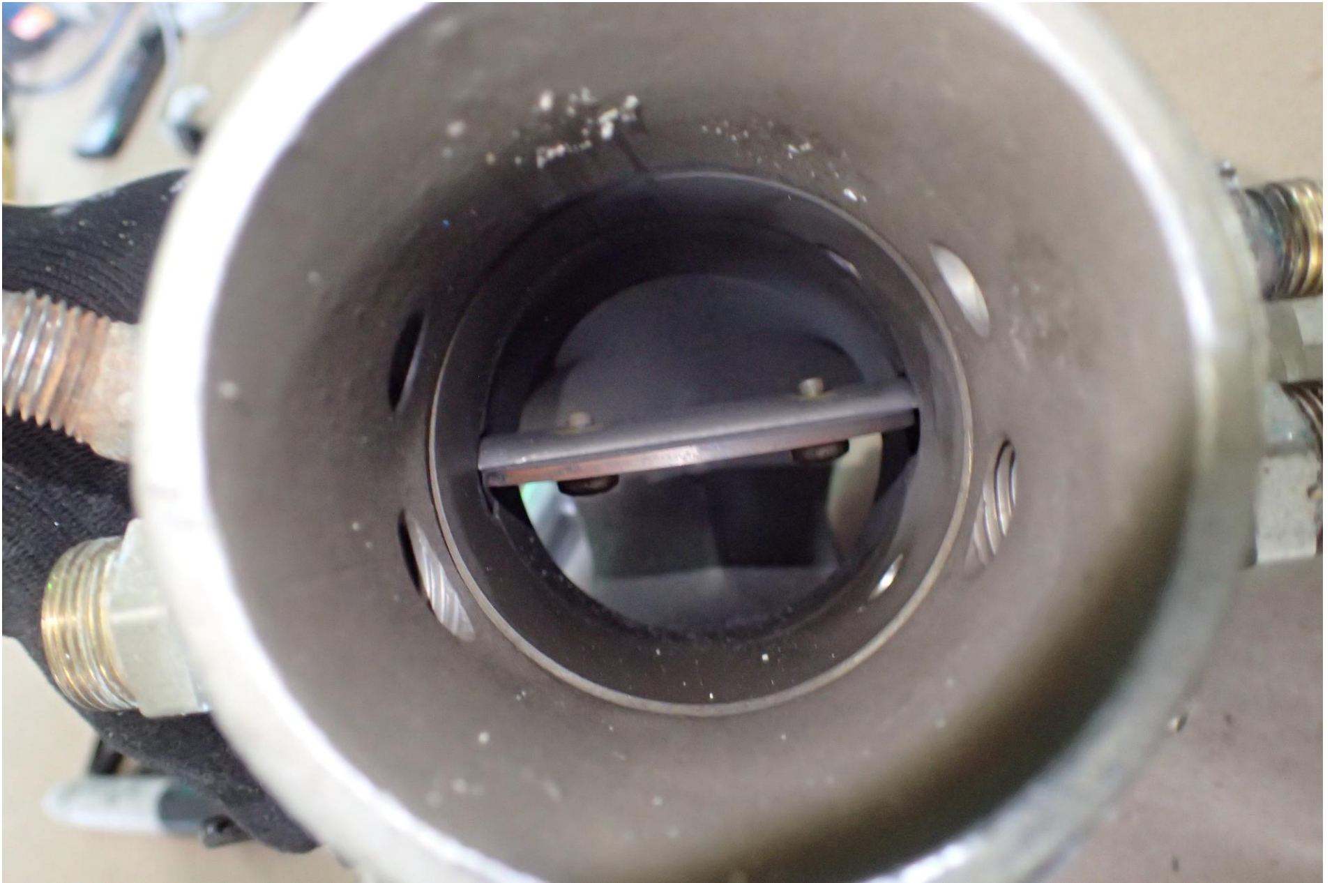
Photo 15 – Fuel Metering Unit (CAT Photo)
