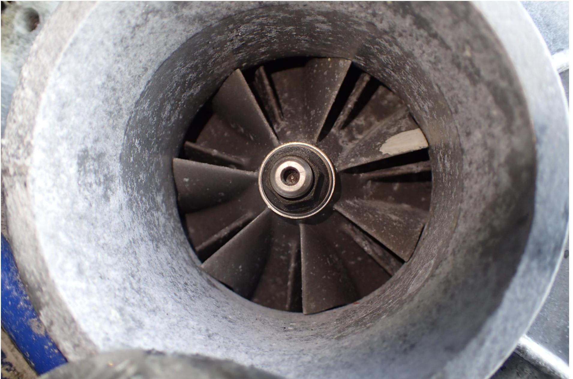
Photo 12 – Turbocharger Inlet (CAT Photo)
