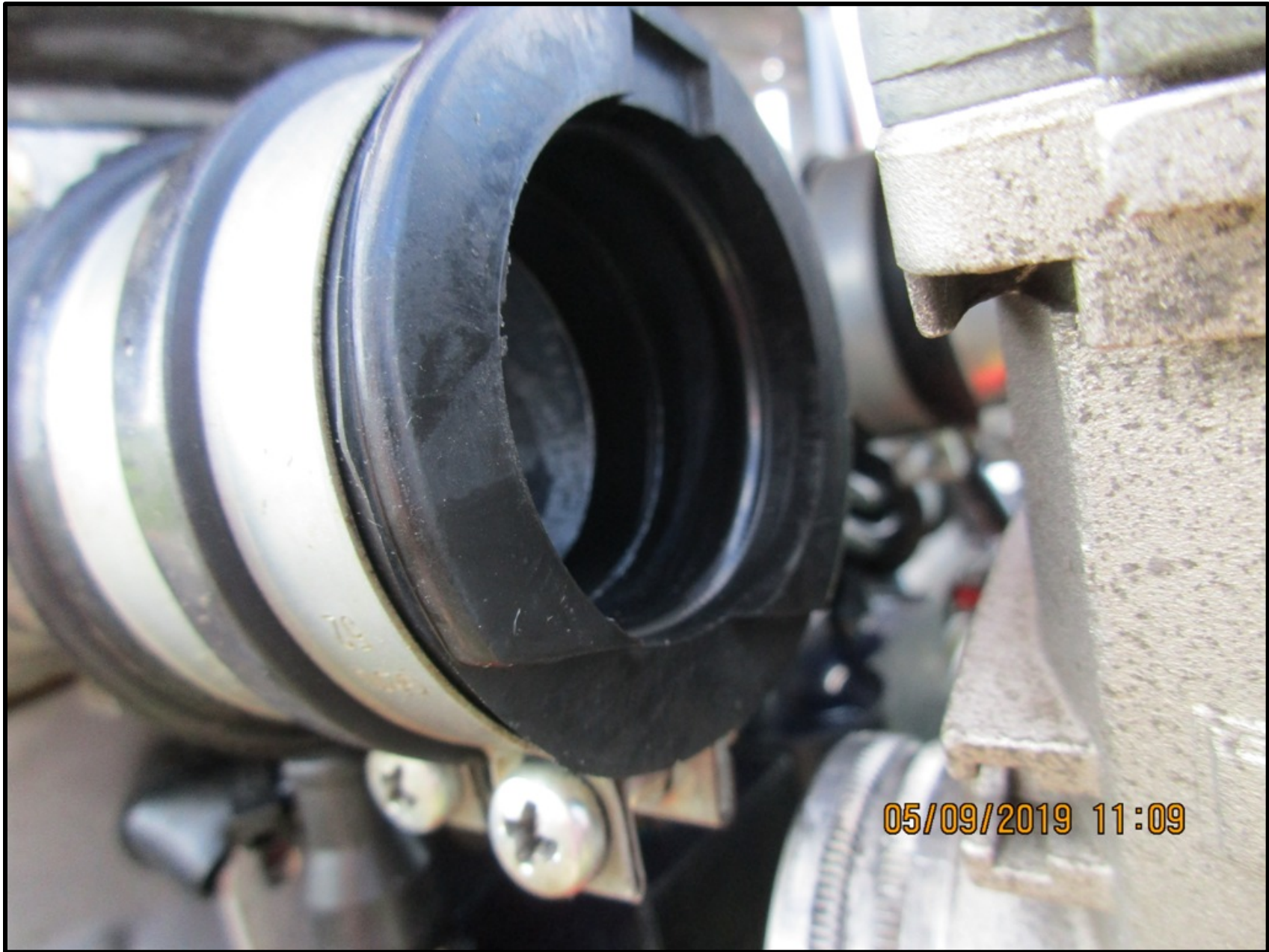
Photo 3 – Forward Carburetor Socket (FAA Photo)
