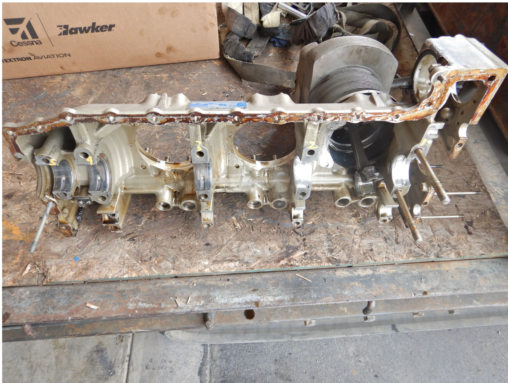
Photo 6 – Engine case half
