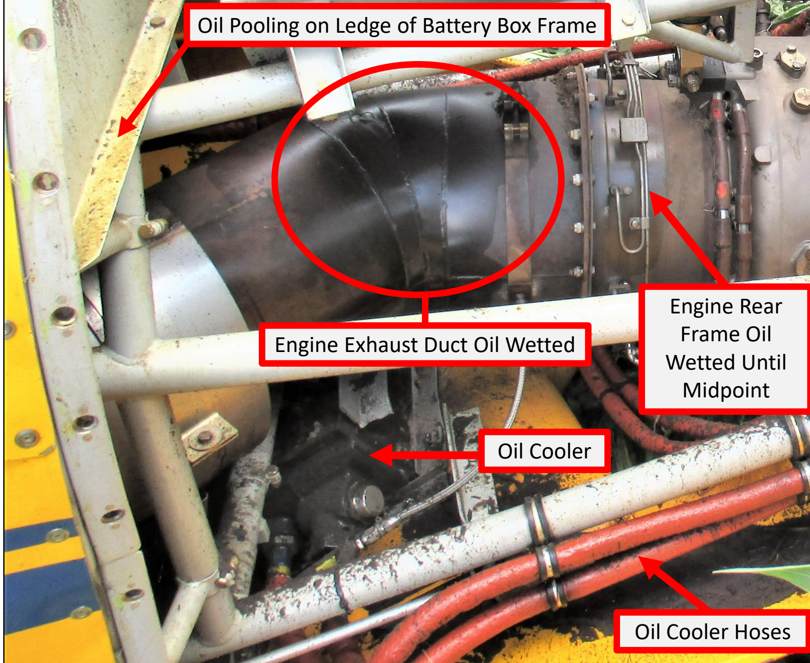
Photo 3 – Engine Exhaust and Oil Cooler (Photo Courtesy of FAA)
