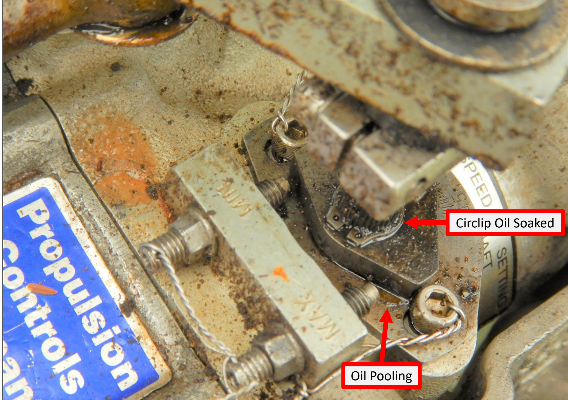
Photo 5 – Fuel Control Unit and Fuel Pump Assembly (Photo Courtesy of Honeywell)
