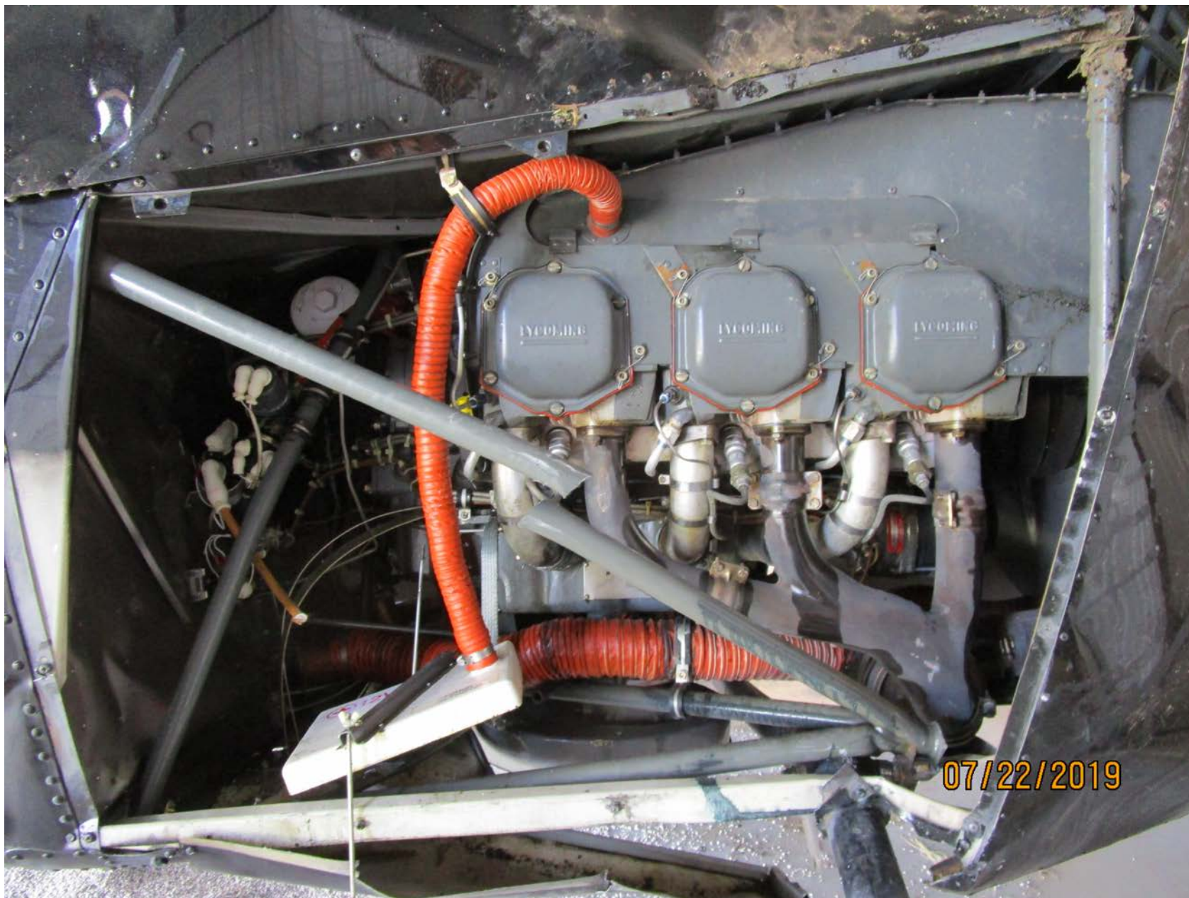
Photo 7 – View of the left side of the engine after it was recovered from the field (courtesy of the Federal Aviation Administration).
