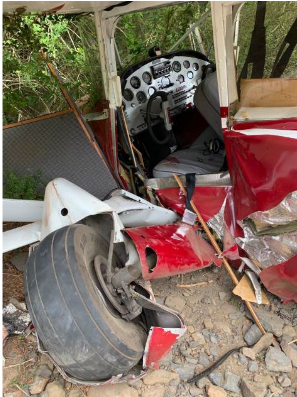
Photo 2 – Cockpit and Fuselage Damage (Photo from Dawson Aircraft)
