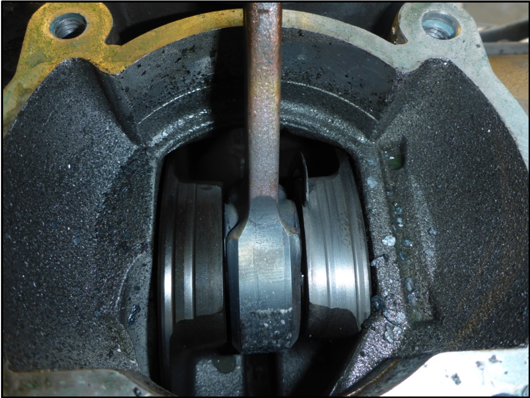
Photo 5 – Connecting Rod
