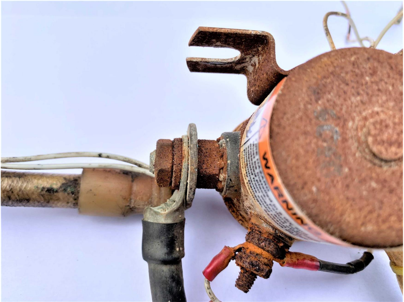
Photo 6 - Battery Contactor Terminal for the Battery Switch and Starter Motor Contactor Cables
