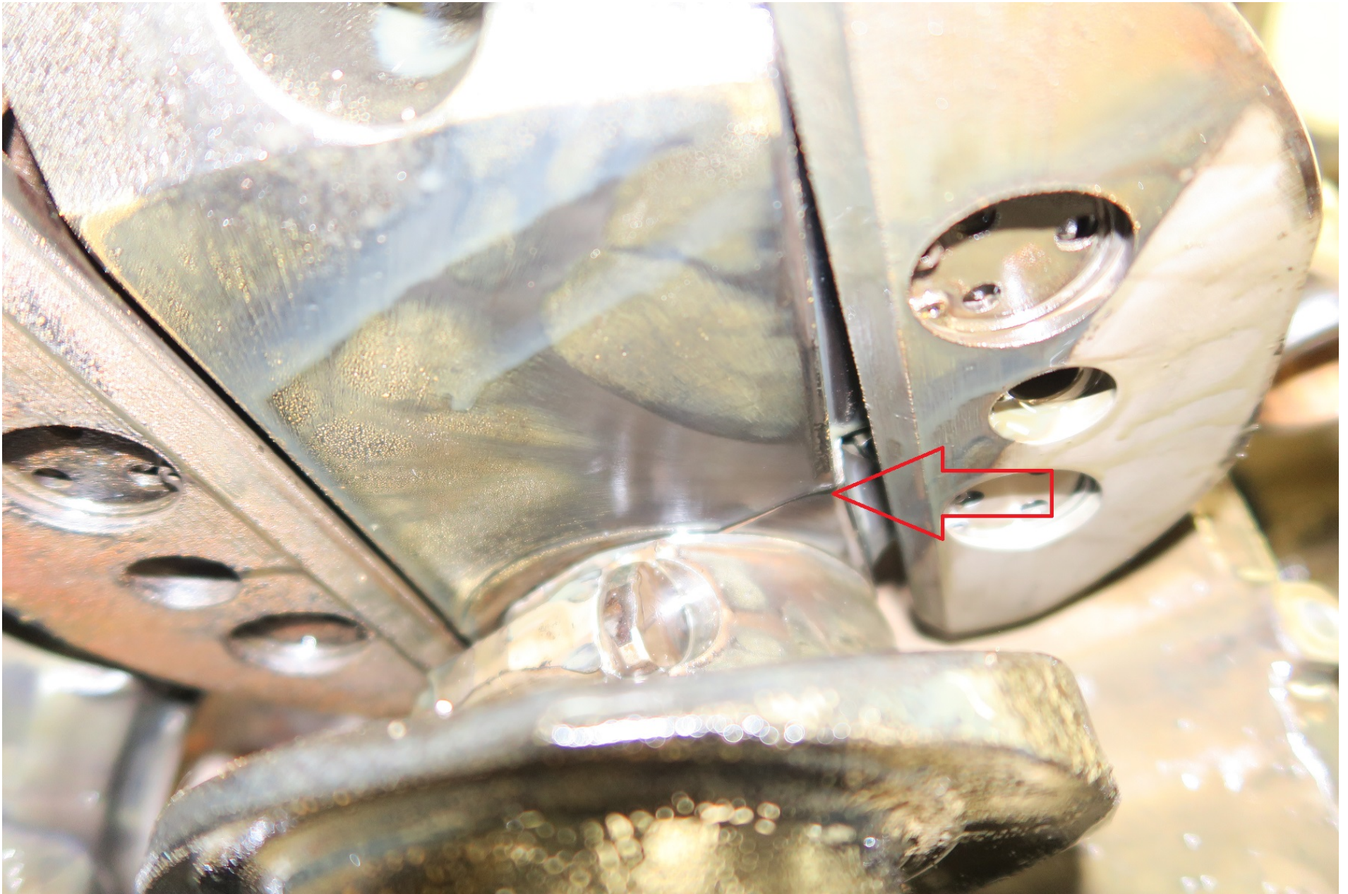
Photo 6 – Crack in crankshaft
