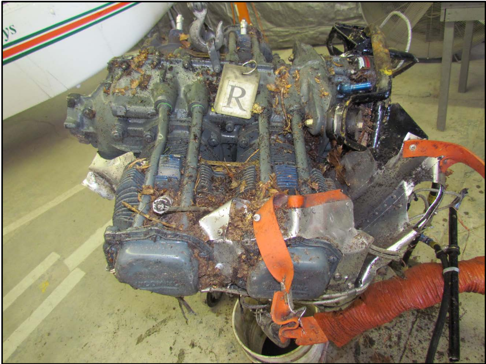
Photo 18 – Right Engine (Lycoming Photo)
