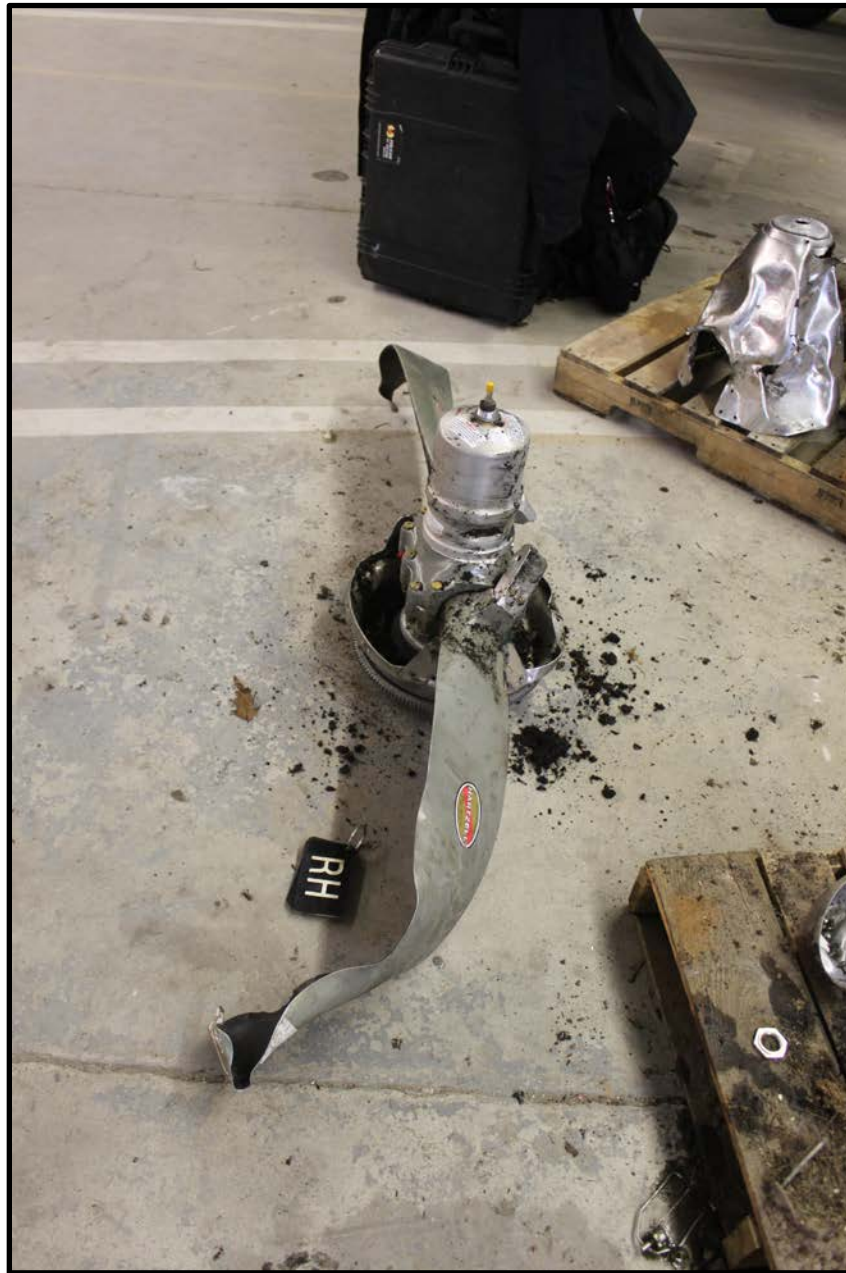
Photo 19 – Right Propeller (NTSB Photo)
