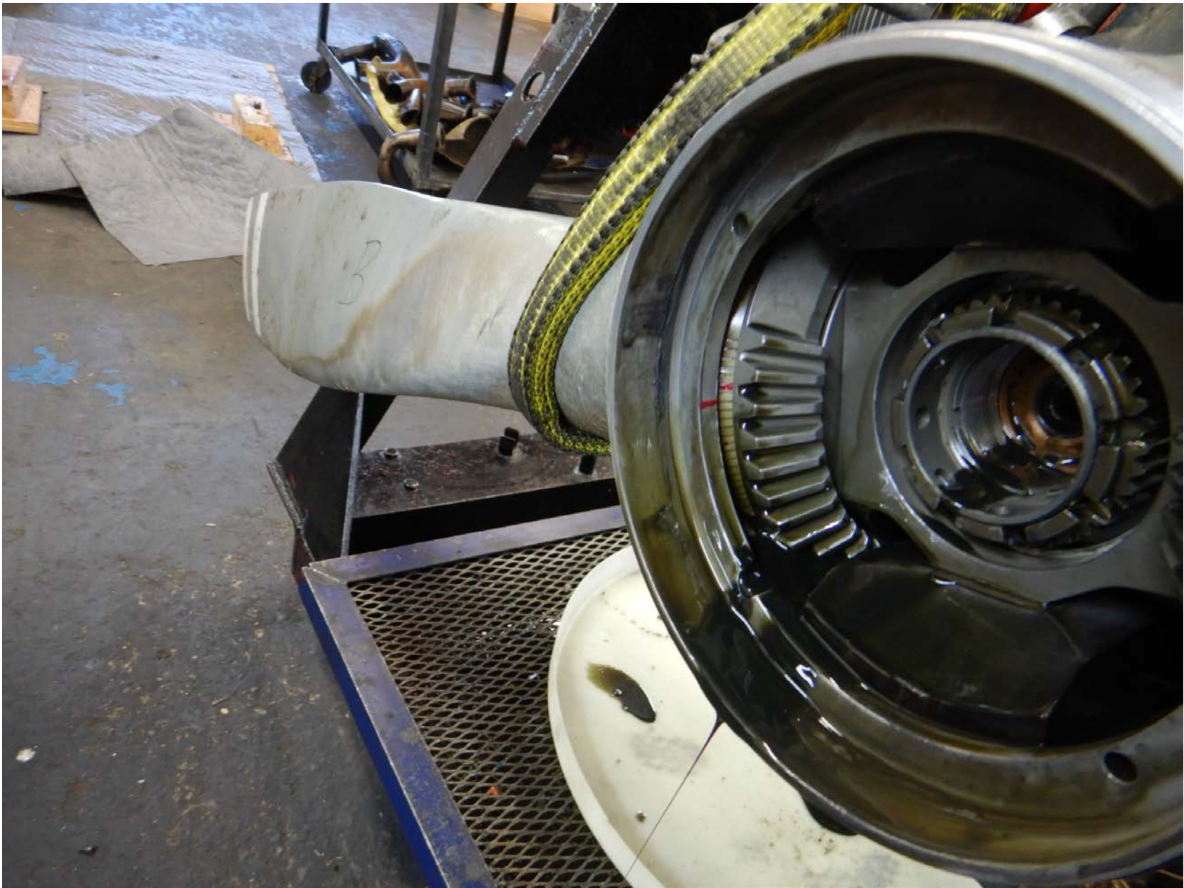
Photo 6 – Propeller “B” Pitch Indication
