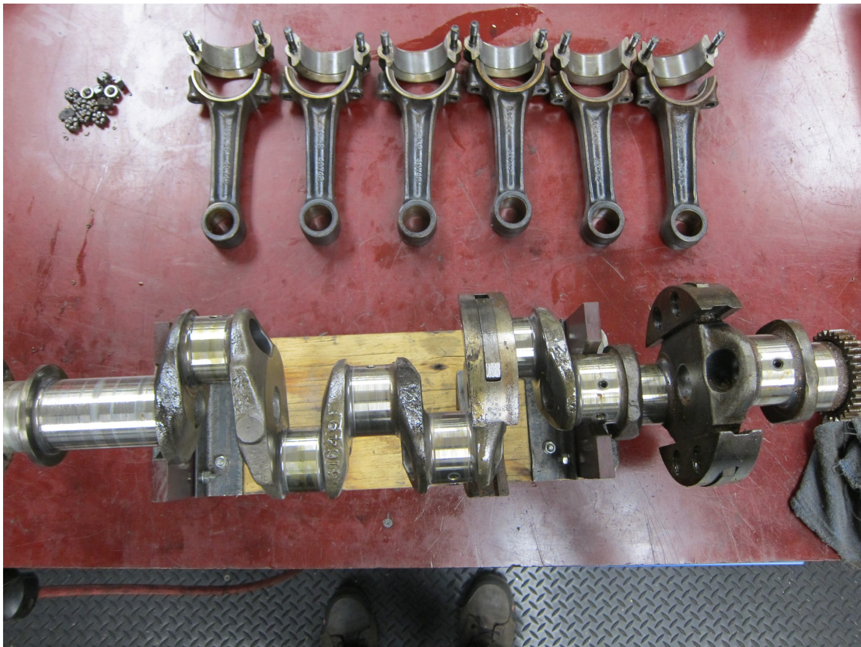
Photo 4 – Crankshaft (CMI Photo)
