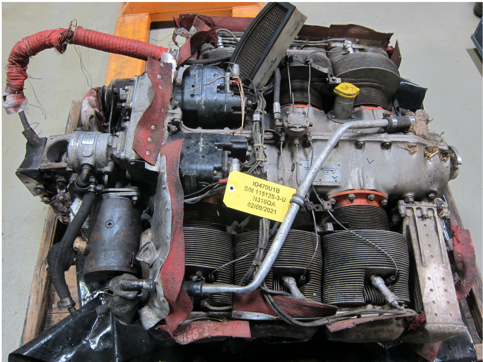
Photo 1 – Engine Overview, Left Engine (CMI Photo)
