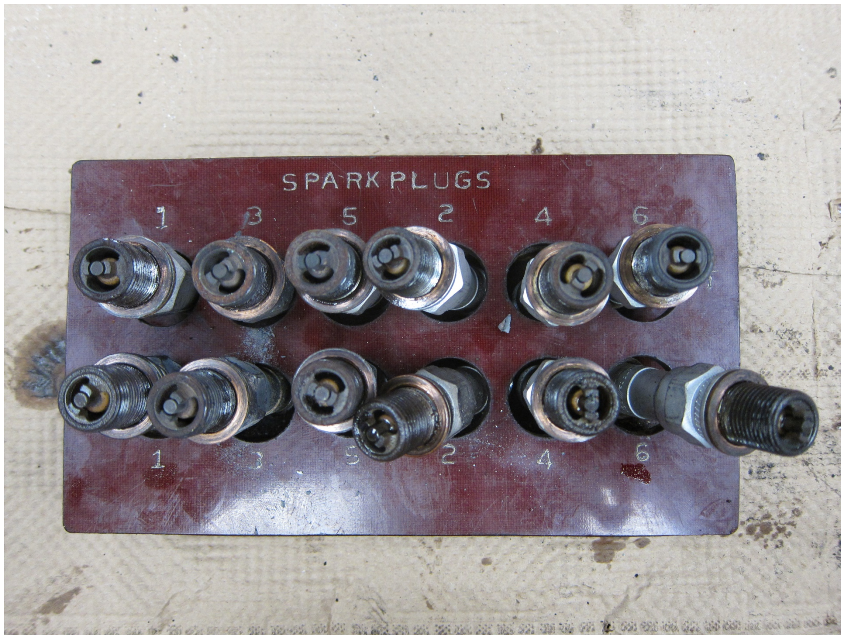
Photo 6 – Spark Plugs (CMI Photo)
