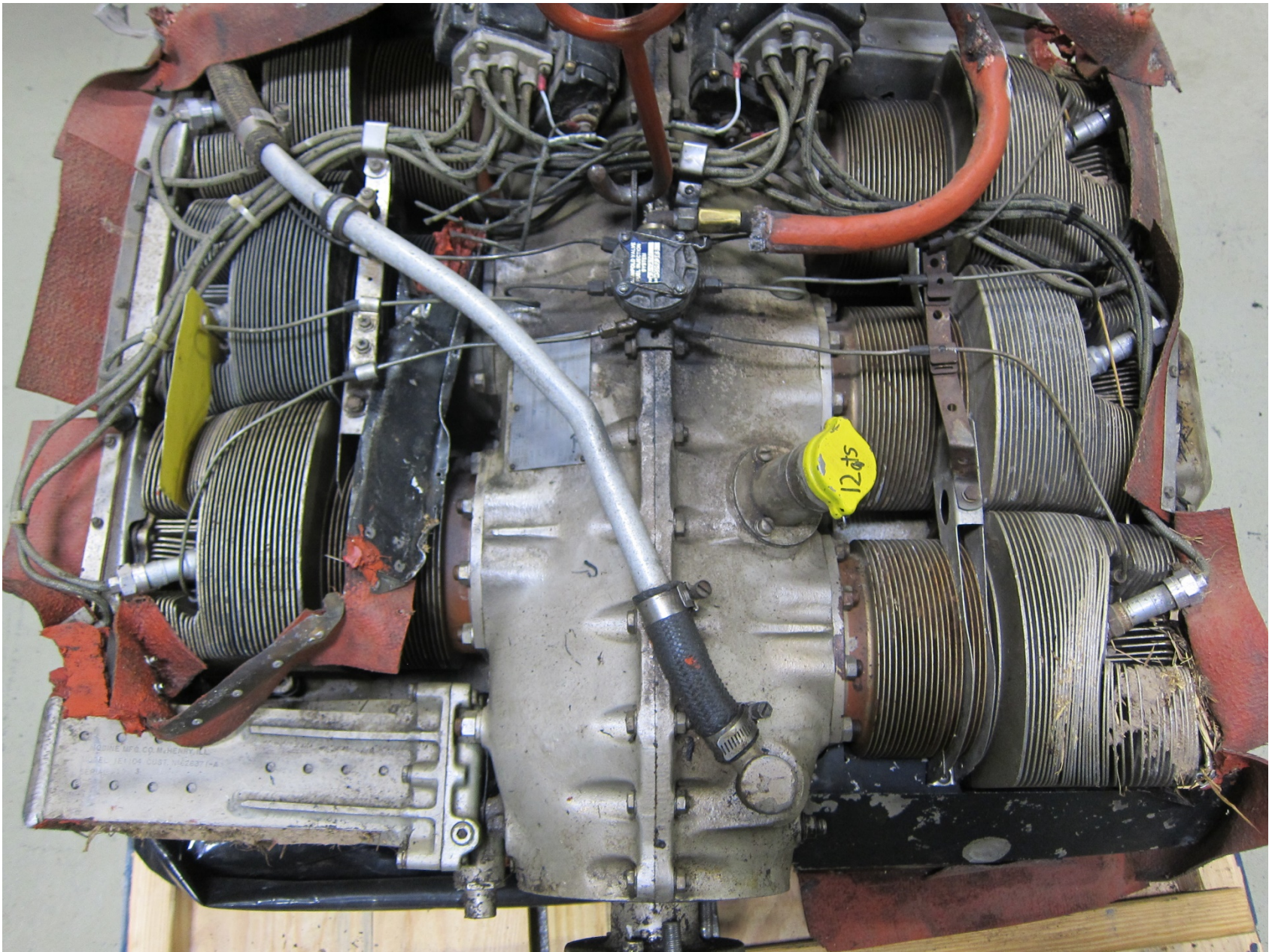
Photo 1 – Engine Overview, Right Engine (CMI Photo)
