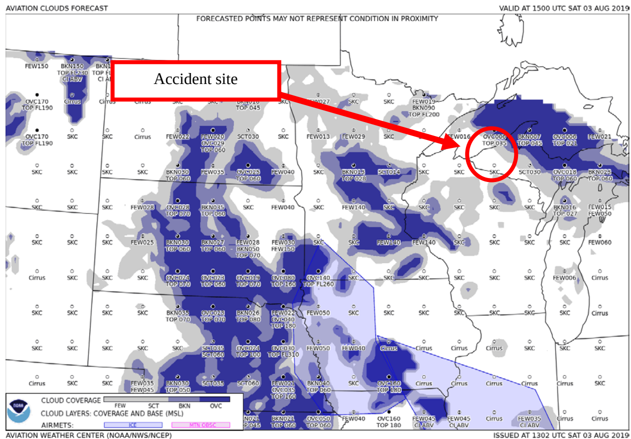
Figure 4 – GFA Aviation Clouds Forecast valid at 1100 EDT with forecast issued at 0902 EDT
