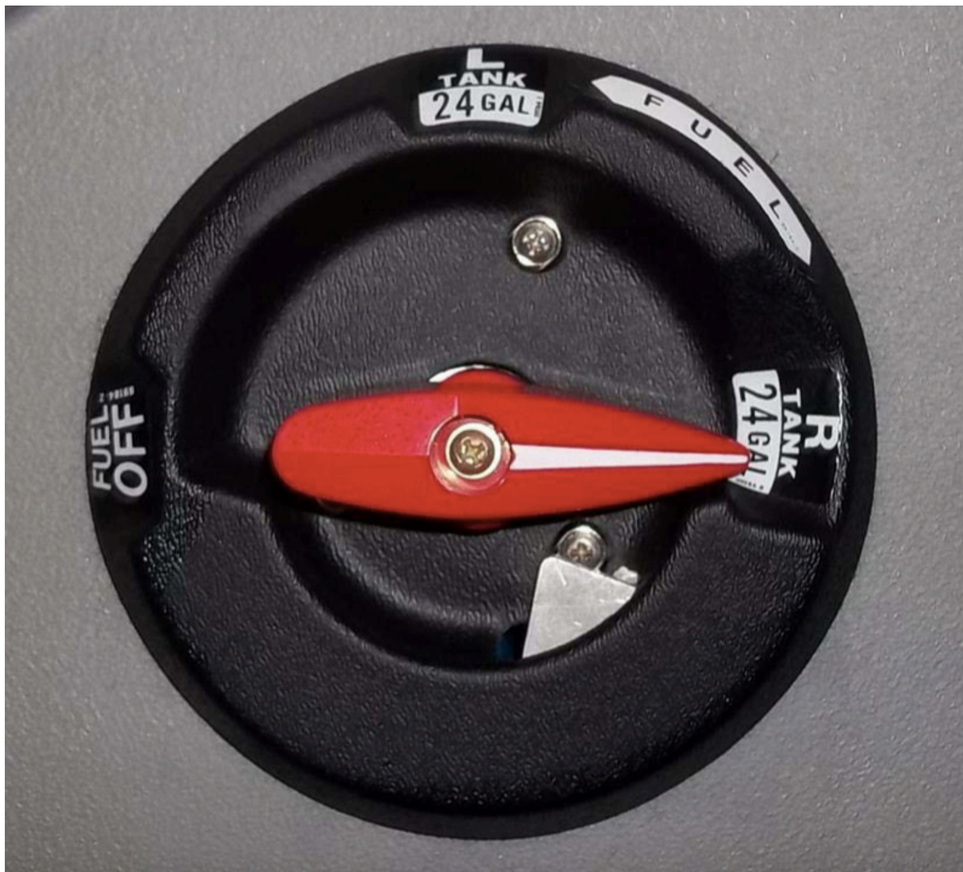
Photo 10 – Exemplar photograph of new style fuel selector
