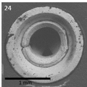
SEM Images of sockets with a nick or deposit at the ~1:00 position—continued
