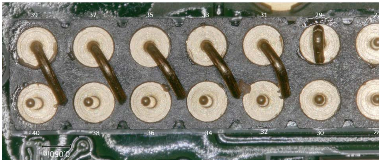
Digital microscope image of the bent pins
