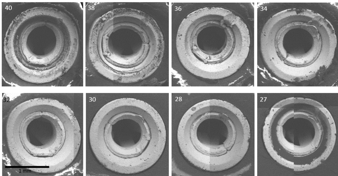
SEM Images of sockets with a nick or deposit at the ~1:00 position
