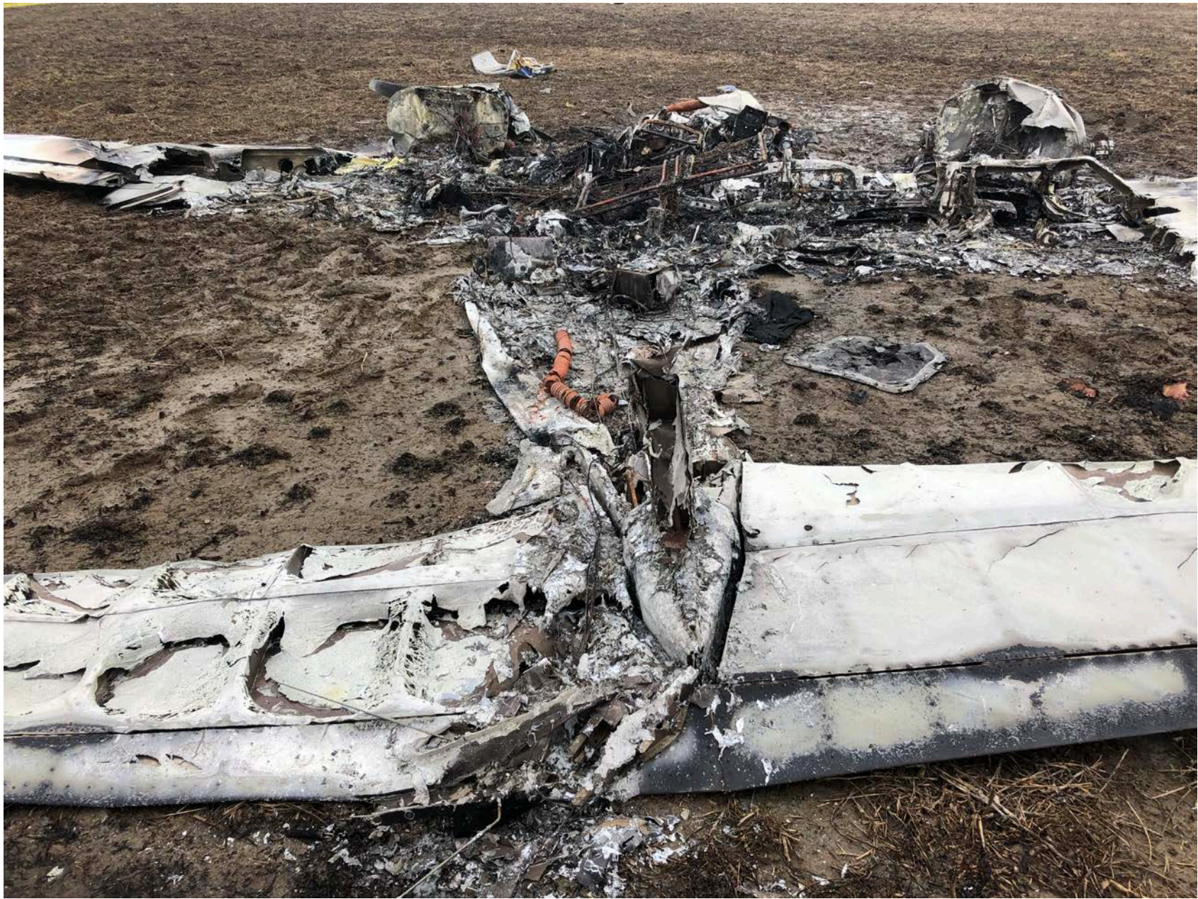
Photo 3 – View of Fuselage
