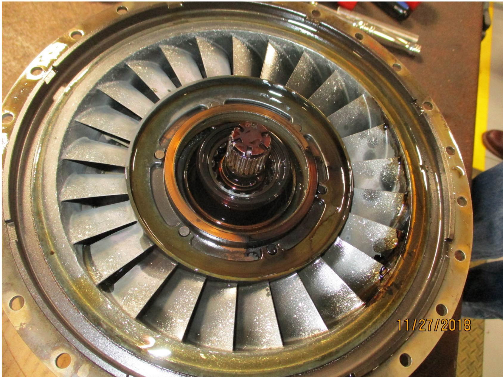
Metal spray is noted on the turbine wheel during engine exam
