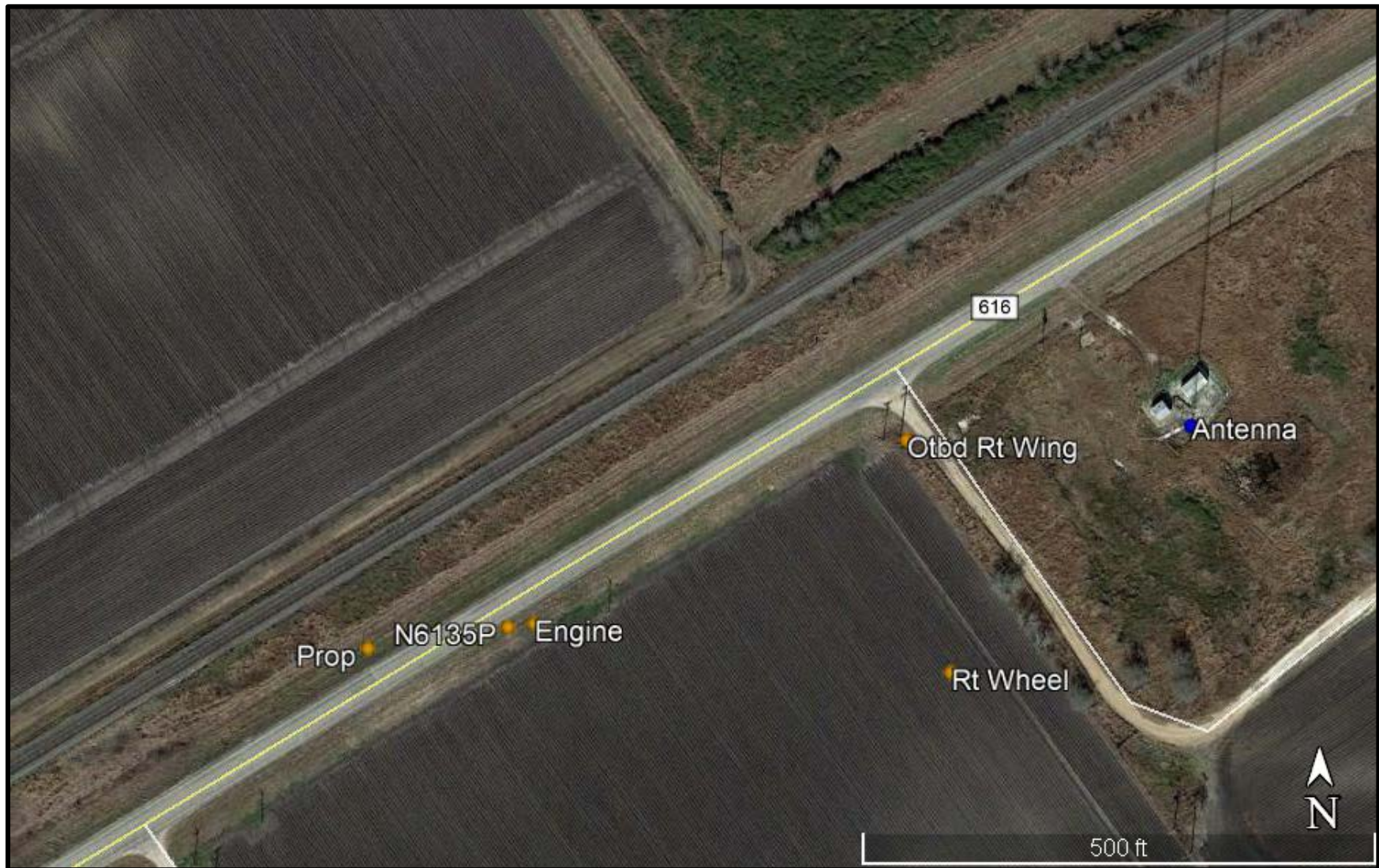
Figure 2 – Wreckage Diagram
