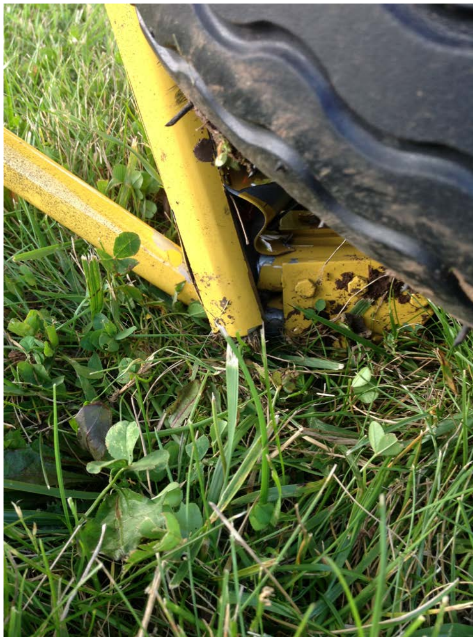
Photograph 03 - Collapsed Left Main Landing Gear
