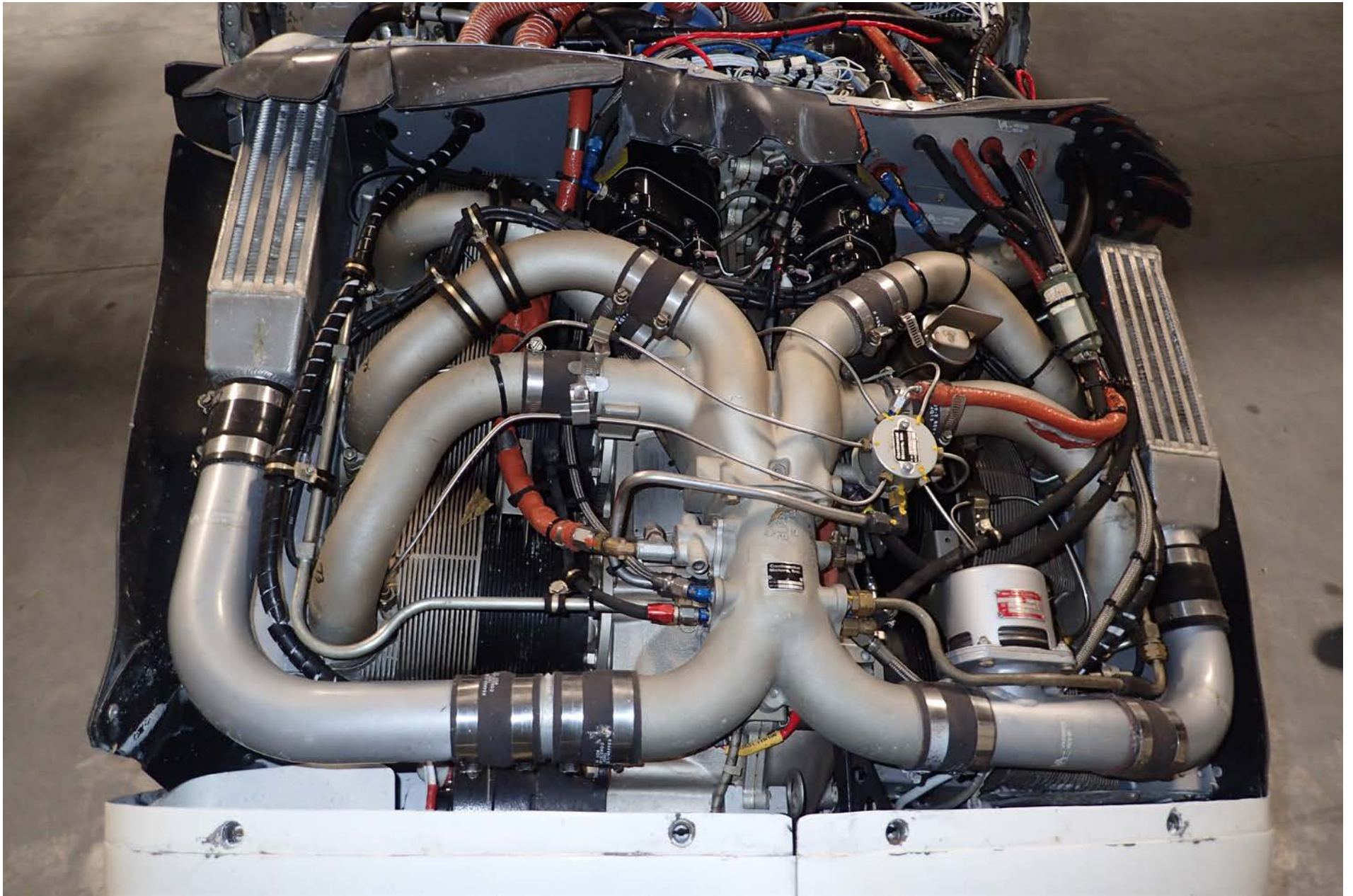
Photo 4 – View of the top of the engine (CM Photo)
